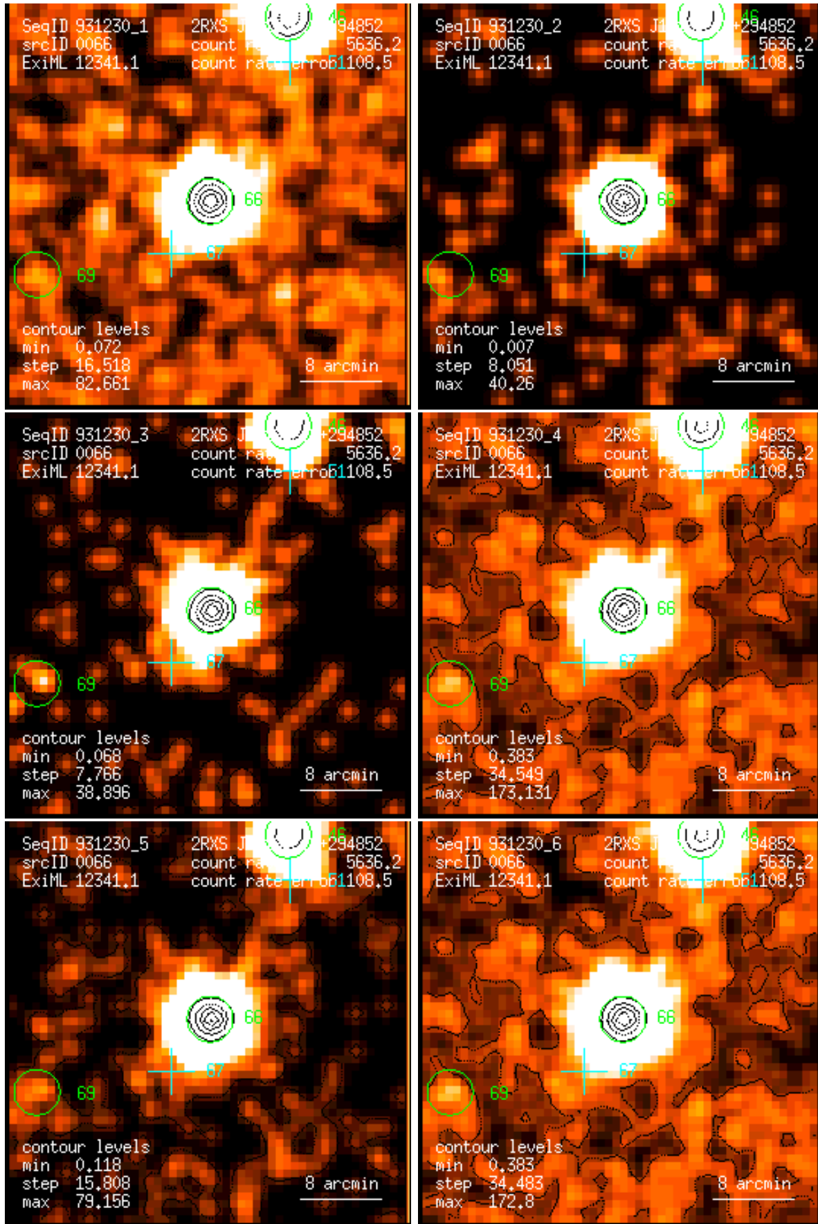
Figure 66: RASS 931230: detection 0066: band rate images, Gaussian filter: (1) PSPC channels 11 – 41, (2) 52 – 90, (3) 91 – 201, (4) 11 – 235, (5) 52 – 201, (6) 11 – 201. Broad band rates in counts/ks. Band rate contour levels in counts/ks/arcmin 2 .
