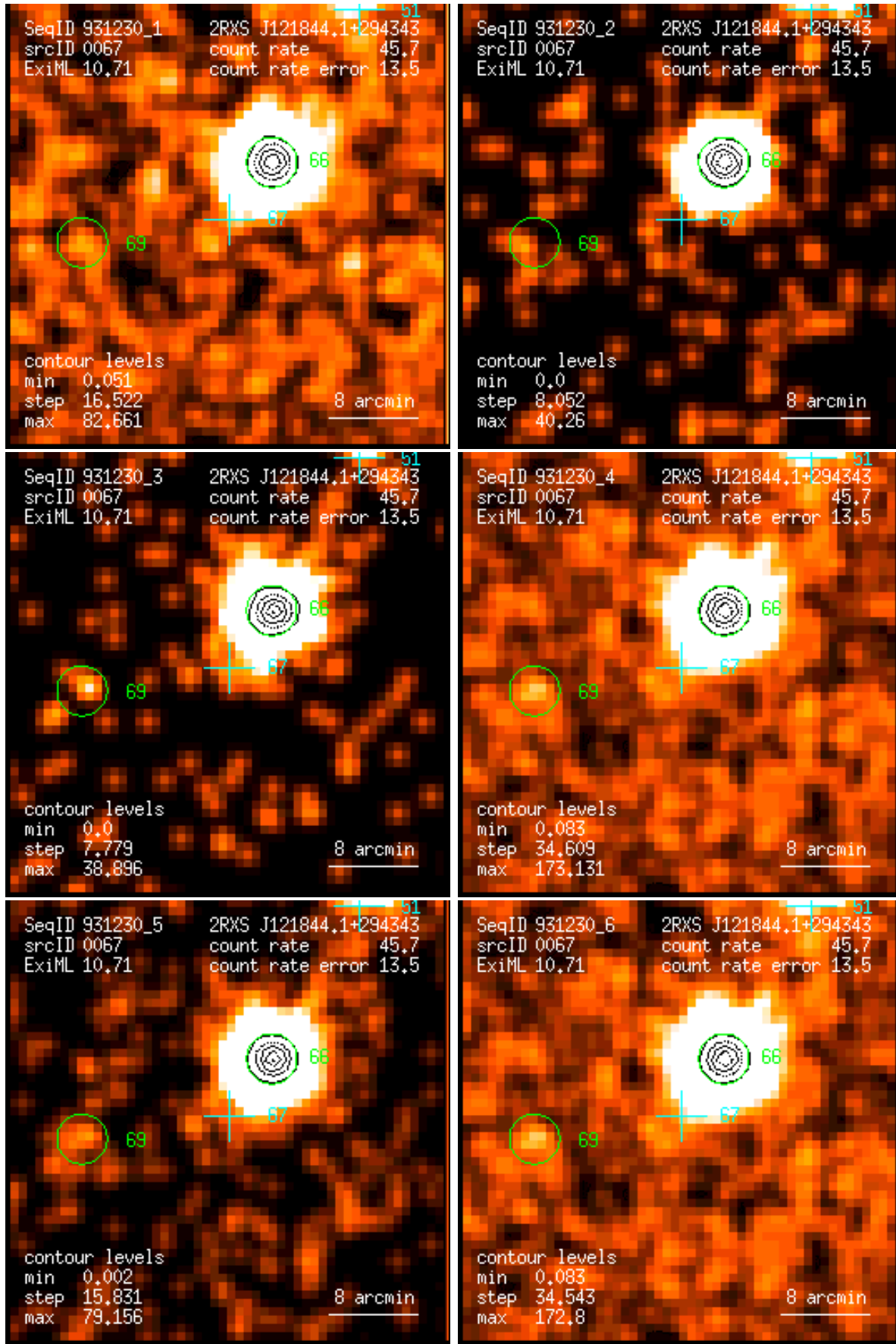
Figure 67: RASS 931230: detection 0067: band rate images, Gaussian filter: (1) PSPC channels 11 – 41, (2) 52 – 90, (3) 91 – 201, (4) 11 – 235, (5) 52 – 201, (6) 11 – 201. Broad band rates in counts/ks. Band rate contour levels in counts/ks/arcmin 2 .
