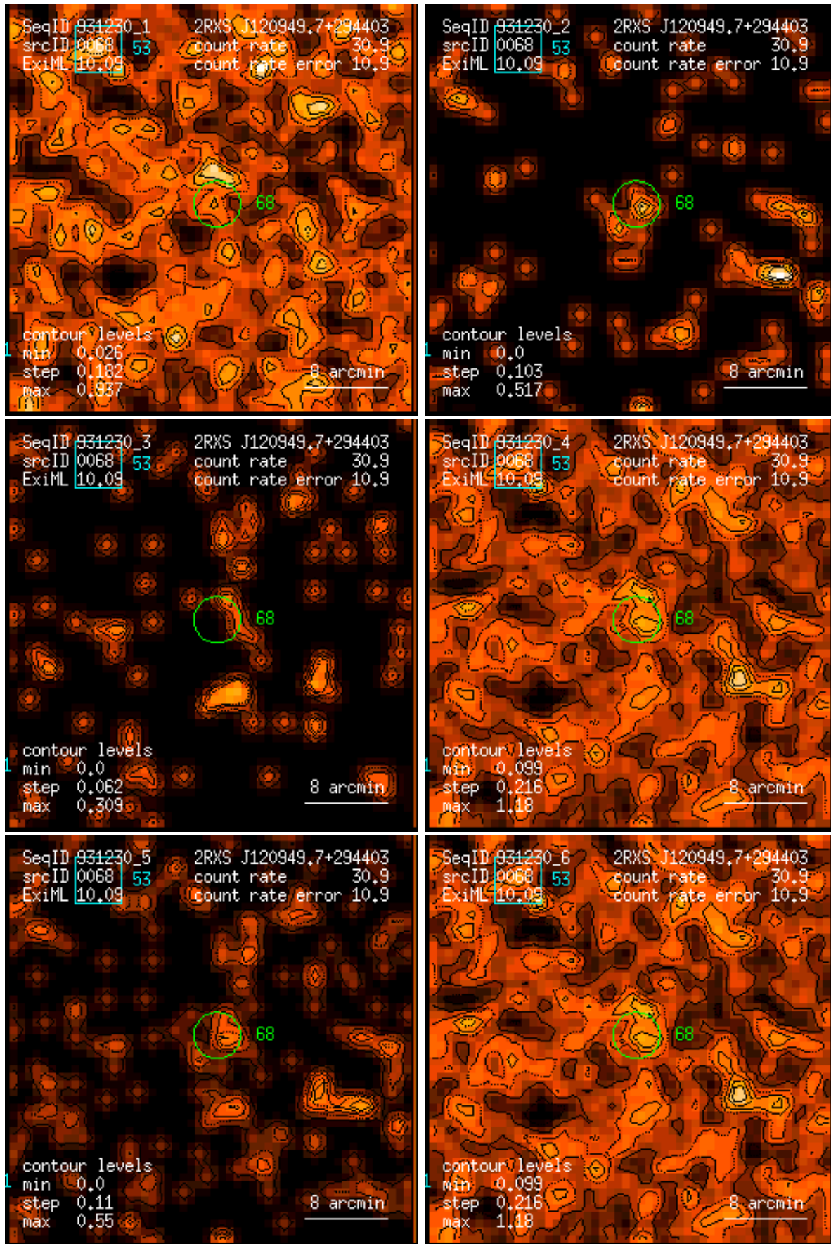
Figure 68: RASS 931230: detection 0068: band rate images, Gaussian filter: (1) PSPC channels 11 – 41, (2) 52 – 90, (3) 91 – 201, (4) 11 – 235, (5) 52 – 201, (6) 11 – 201. Broad band rates in counts/ks. Band rate contour levels in counts/ks/arcmin 2 .
