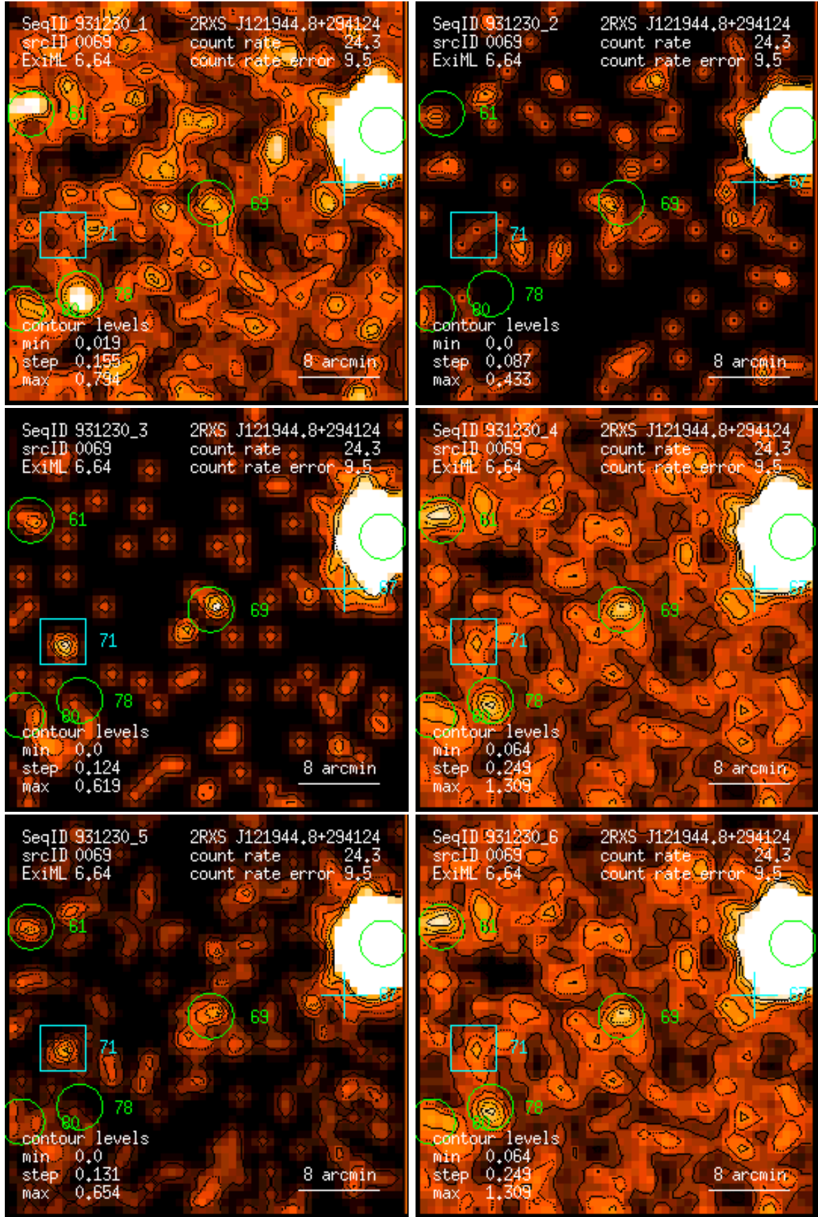
Figure 69: RASS 931230: detection 0069: band rate images, Gaussian filter: (1) PSPC channels 11 – 41, (2) 52 – 90, (3) 91 – 201, (4) 11 – 235, (5) 52 – 201, (6) 11 – 201. Broad band rates in counts/ks. Band rate contour levels in counts/ks/arcmin 2 .
