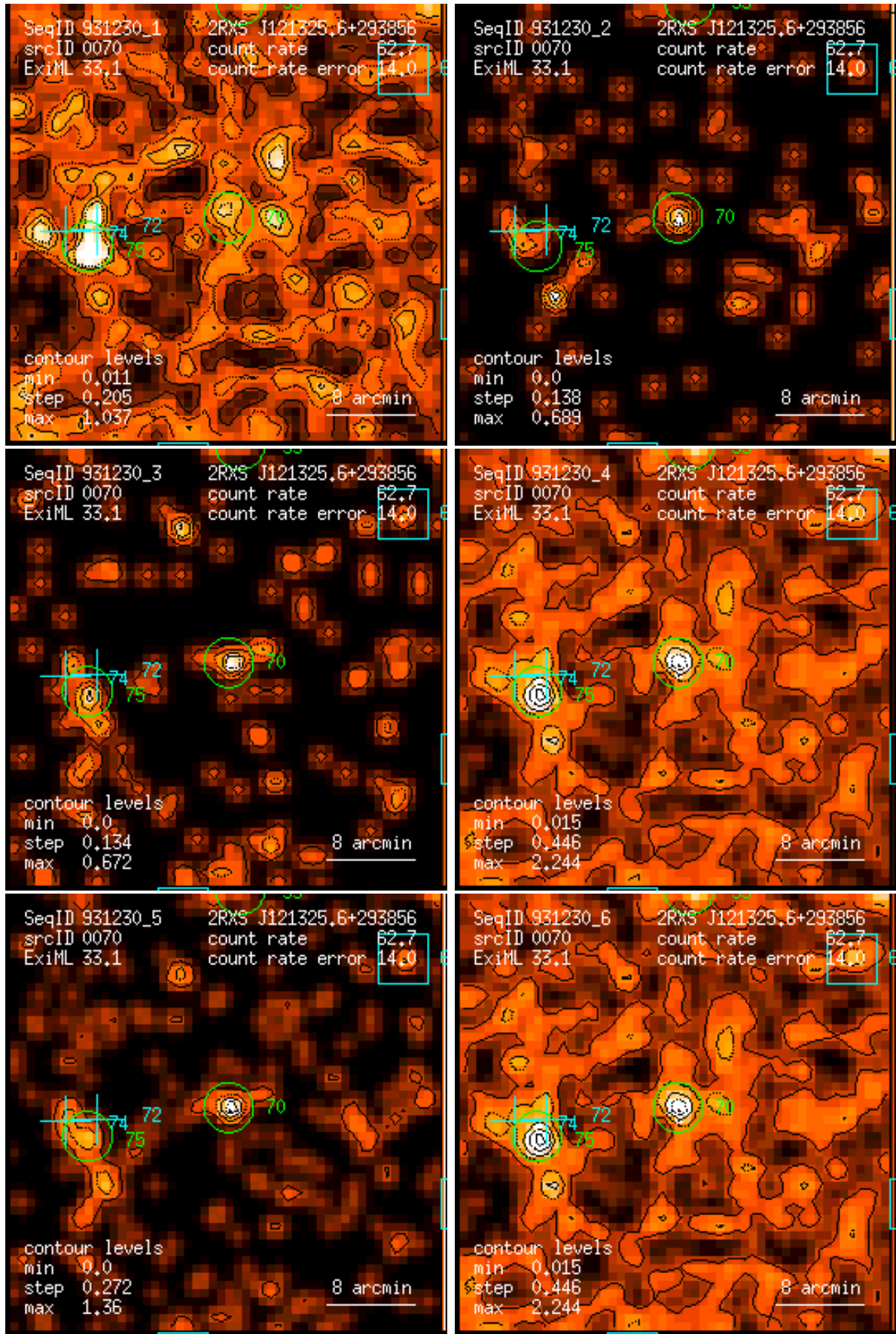
Figure 70: RASS 931230: detection 0070: band rate images, Gaussian filter: (1) PSPC channels 11 – 41, (2) 52 – 90, (3) 91 – 201, (4) 11 – 235, (5) 52 – 201, (6) 11 – 201. Broad band rates in counts/ks. Band rate contour levels in counts/ks/arcmin 2 .
