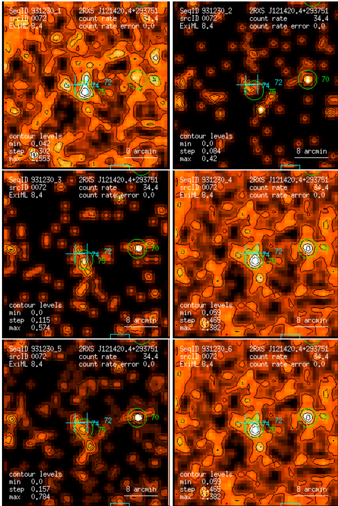
Figure 72: RASS 931230: detection 0072: band rate images, Gaussian filter: (1) PSPC channels 11 – 41, (2) 52 – 90, (3) 91 – 201, (4) 11 – 235, (5) 52 – 201, (6) 11 – 201. Broad band rates in counts/ks. Band rate contour levels in counts/ks/arcmin 2 .
