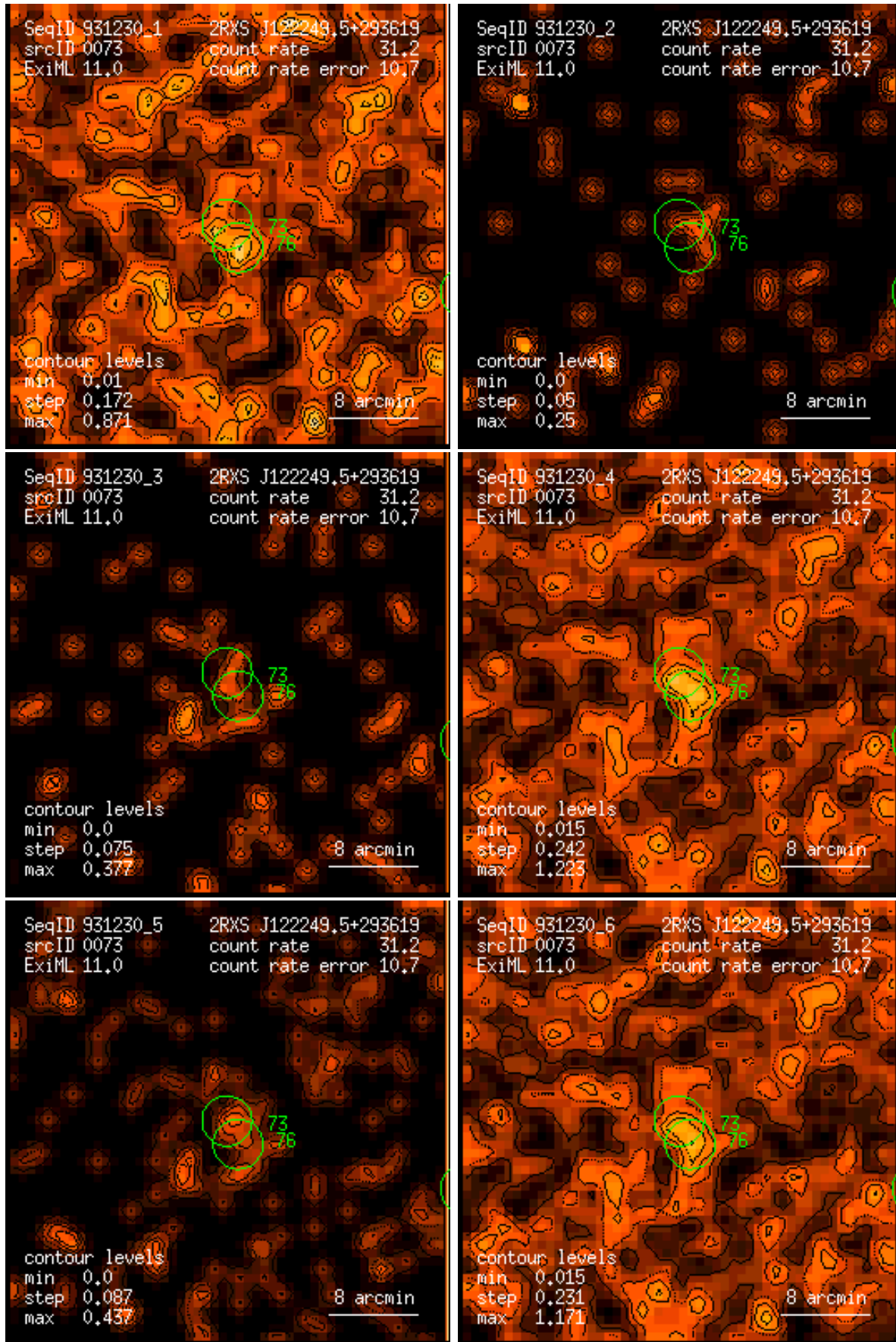
Figure 73: RASS 931230: detection 0073: band rate images, Gaussian filter: (1) PSPC channels 11 – 41, (2) 52 – 90, (3) 91 – 201, (4) 11 – 235, (5) 52 – 201, (6) 11 – 201. Broad band rates in counts/ks. Band rate contour levels in counts/ks/arcmin 2 .
