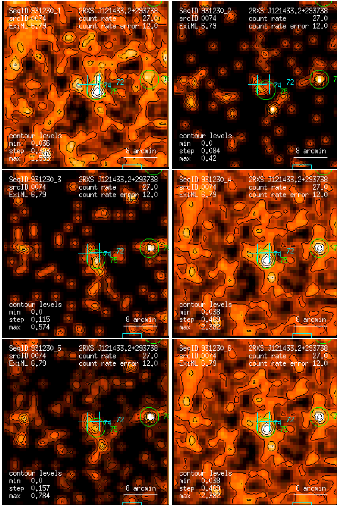
Figure 74: RASS 931230: detection 0074: band rate images, Gaussian filter: (1) PSPC channels 11 – 41, (2) 52 – 90, (3) 91 – 201, (4) 11 – 235, (5) 52 – 201, (6) 11 – 201. Broad band rates in counts/ks. Band rate contour levels in counts/ks/arcmin 2 .
