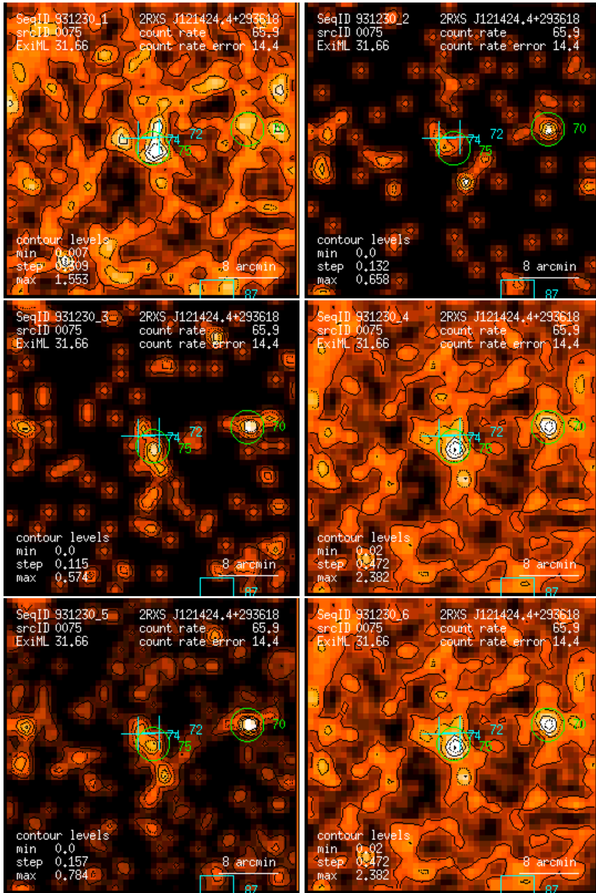
Figure 75: RASS 931230: detection 0075: band rate images, Gaussian filter: (1) PSPC channels 11 – 41, (2) 52 – 90, (3) 91 – 201, (4) 11 – 235, (5) 52 – 201, (6) 11 – 201. Broad band rates in counts/ks. Band rate contour levels in counts/ks/arcmin 2 .
