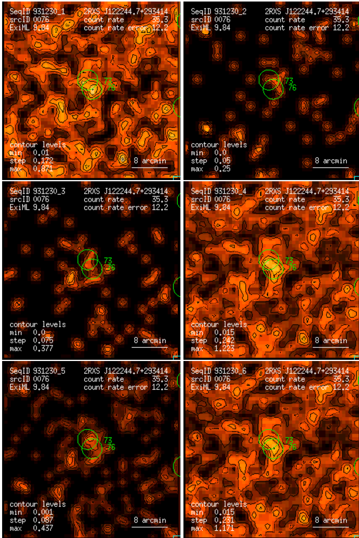
Figure 76: RASS 931230: detection 0076: band rate images, Gaussian filter: (1) PSPC channels 11 – 41, (2) 52 – 90, (3) 91 – 201, (4) 11 – 235, (5) 52 – 201, (6) 11 – 201. Broad band rates in counts/ks. Band rate contour levels in counts/ks/arcmin 2 .
