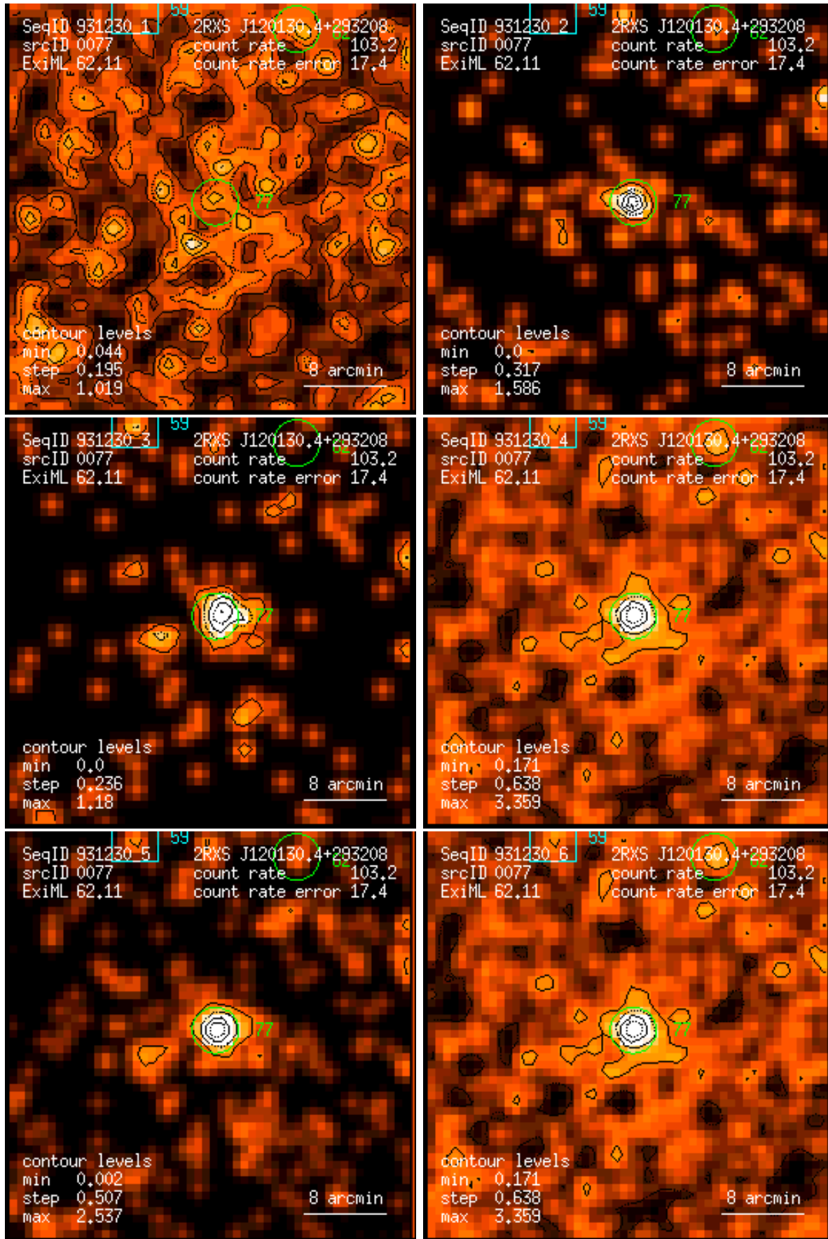
Figure 77: RASS 931230: detection 0077: band rate images, Gaussian filter: (1) PSPC channels 11 – 41, (2) 52 – 90, (3) 91 – 201, (4) 11 – 235, (5) 52 – 201, (6) 11 – 201. Broad band rates in counts/ks. Band rate contour levels in counts/ks/arcmin 2 .
