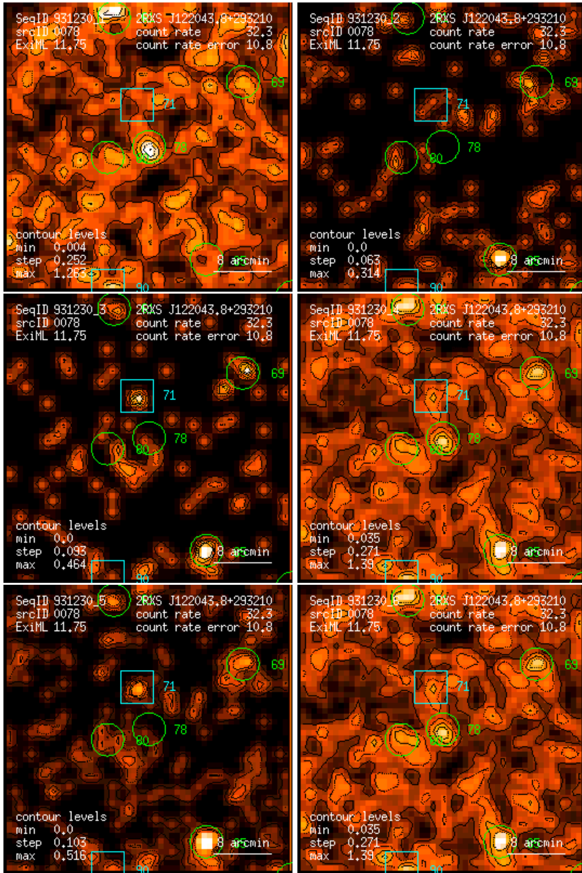
Figure 78: RASS 931230: detection 0078: band rate images, Gaussian filter: (1) PSPC channels 11 – 41, (2) 52 – 90, (3) 91 – 201, (4) 11 – 235, (5) 52 – 201, (6) 11 – 201. Broad band rates in counts/ks. Band rate contour levels in counts/ks/arcmin 2 .
