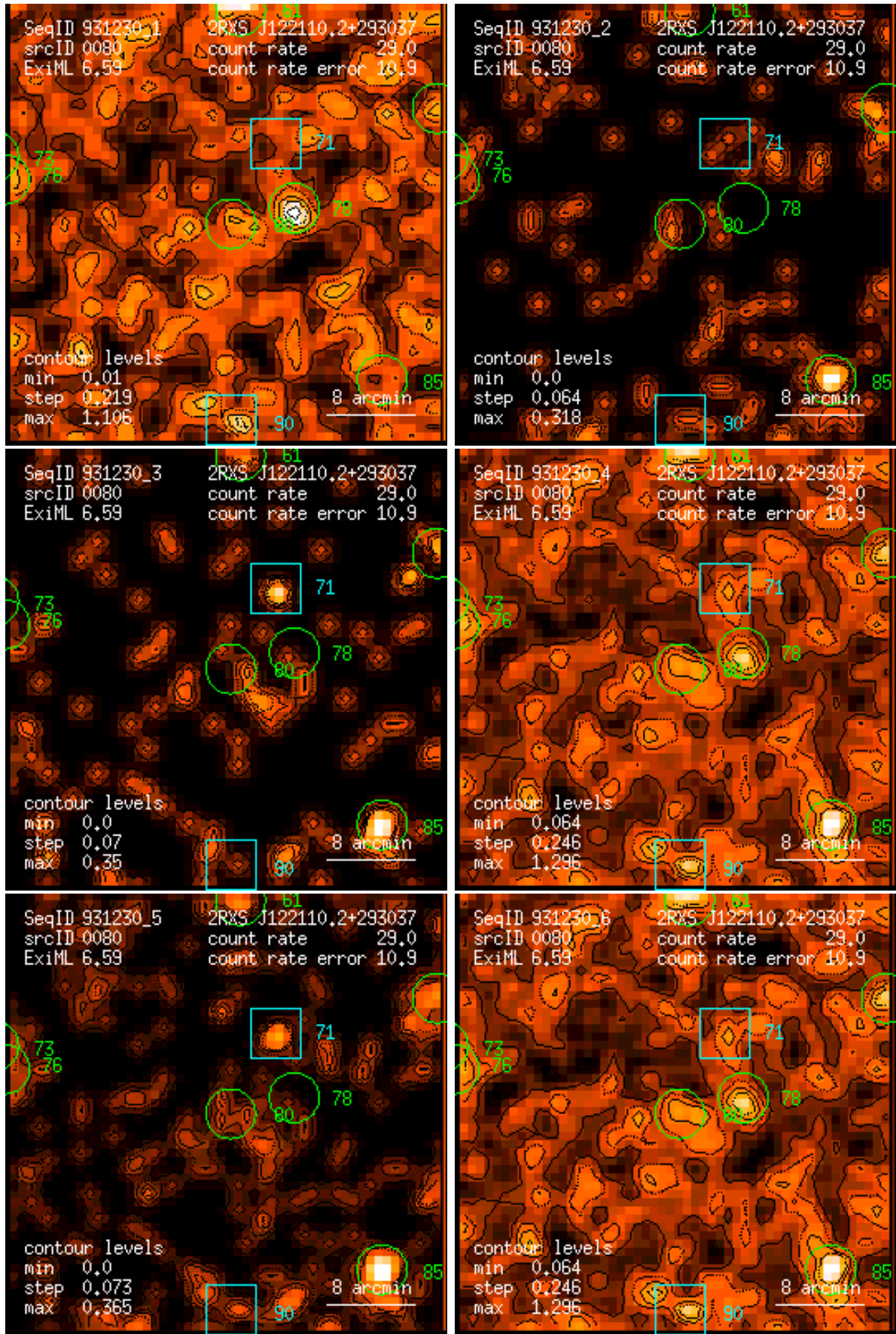
Figure 80: RASS 931230: detection 0080: band rate images, Gaussian filter: (1) PSPC channels 11 – 41, (2) 52 – 90, (3) 91 – 201, (4) 11 – 235, (5) 52 – 201, (6) 11 – 201. Broad band rates in counts/ks. Band rate contour levels in counts/ks/arcmin 2 .
