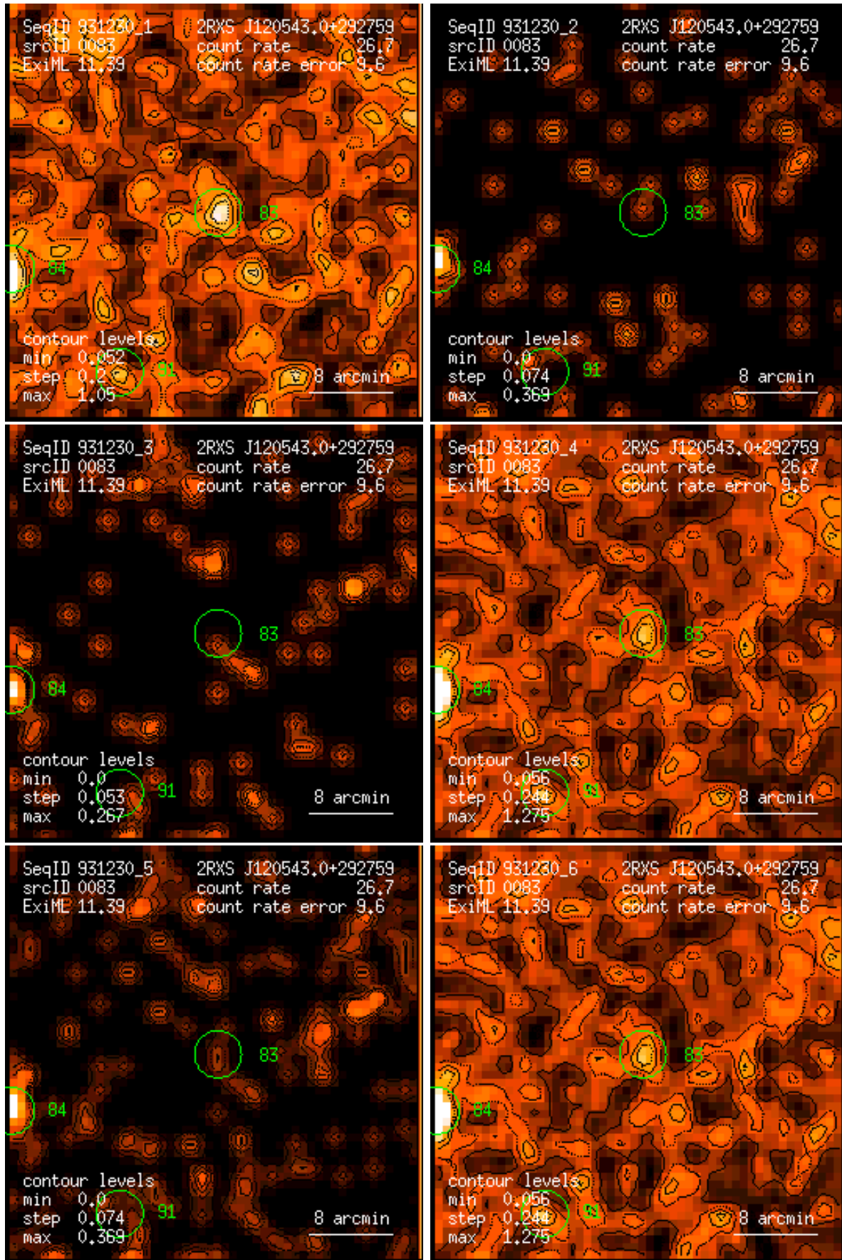
Figure 83: RASS 931230: detection 0083: band rate images, Gaussian filter: (1) PSPC channels 11 – 41, (2) 52 – 90, (3) 91 – 201, (4) 11 – 235, (5) 52 – 201, (6) 11 – 201. Broad band rates in counts/ks. Band rate contour levels in counts/ks/arcmin 2 .
