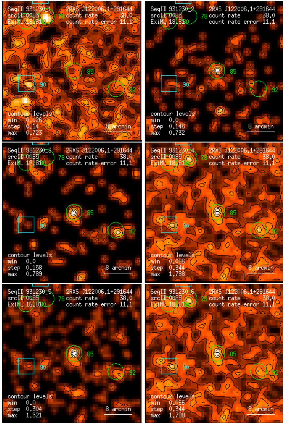
Figure 85: RASS 931230: detection 0085: band rate images, Gaussian filter: (1) PSPC channels 11 – 41, (2) 52 – 90, (3) 91 – 201, (4) 11 – 235, (5) 52 – 201, (6) 11 – 201. Broad band rates in counts/ks. Band rate contour levels in counts/ks/arcmin 2 .
