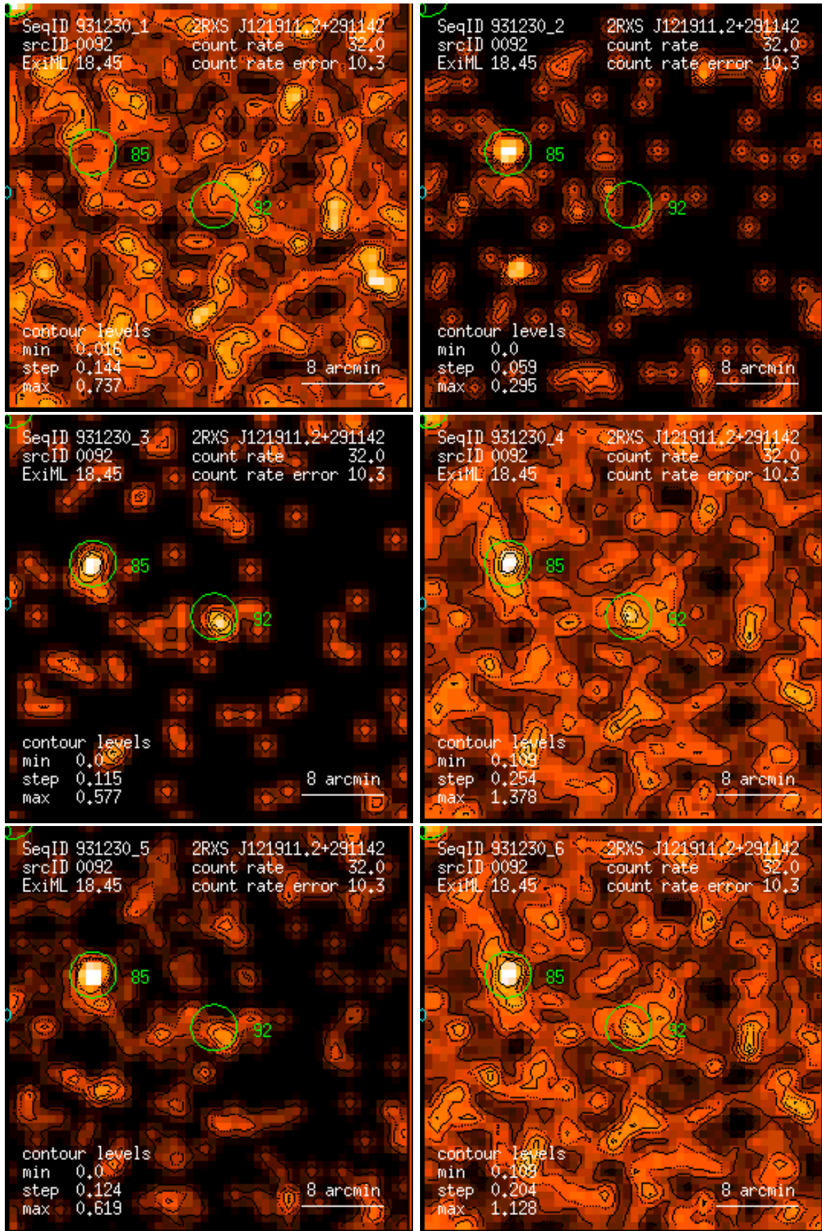
Figure 92: RASS 931230: detection 0092: band rate images, Gaussian filter: (1) PSPC channels 11 – 41, (2) 52 – 90, (3) 91 – 201, (4) 11 – 235, (5) 52 – 201, (6) 11 – 201. Broad band rates in counts/ks. Band rate contour levels in counts/ks/arcmin 2 .
