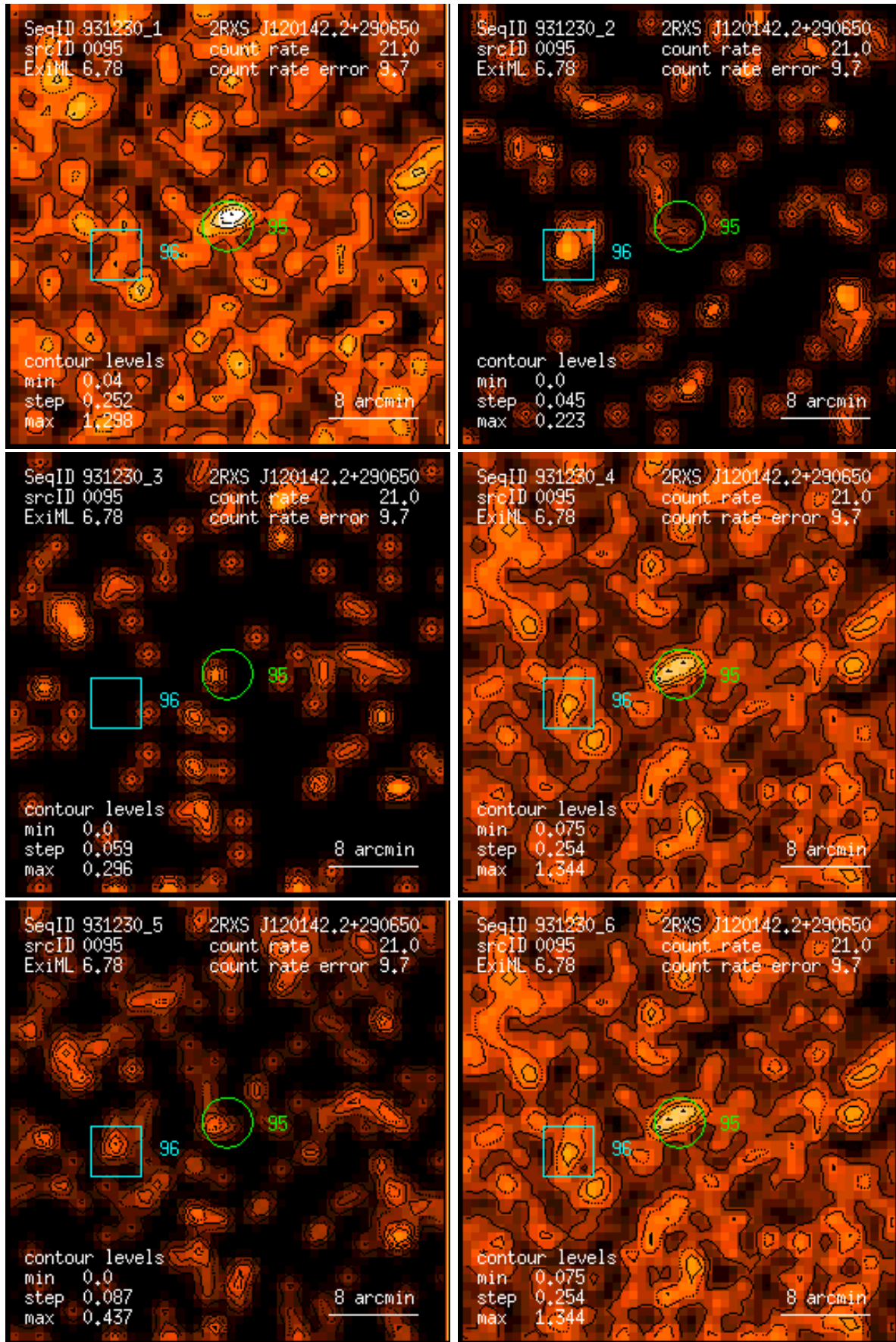
Figure 95: RASS 931230: detection 0095: band rate images, Gaussian filter: (1) PSPC channels 11 – 41, (2) 52 – 90, (3) 91 – 201, (4) 11 – 235, (5) 52 – 201, (6) 11 – 201. Broad band rates in counts/ks. Band rate contour levels in counts/ks/arcmin 2 .
