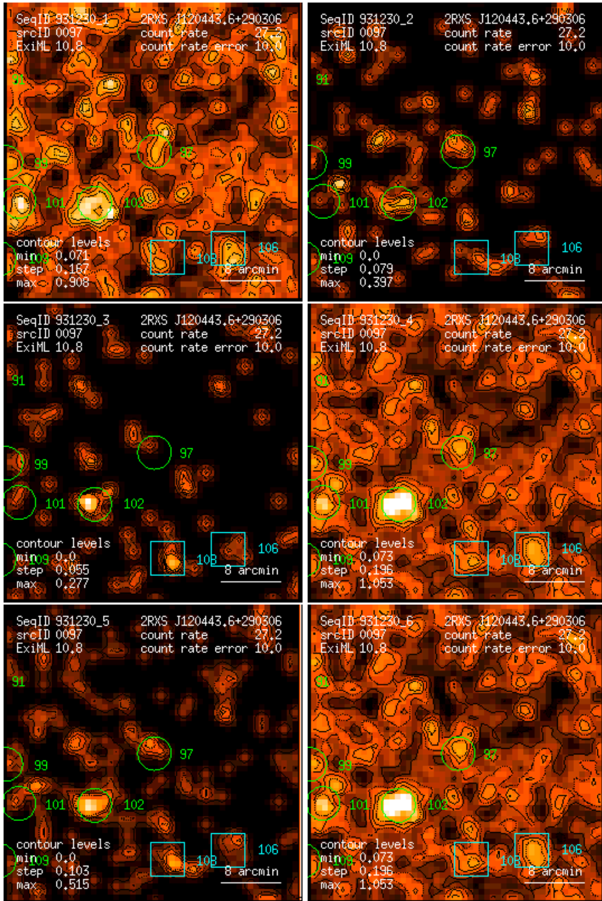
Figure 97: RASS 931230: detection 0097: band rate images, Gaussian filter: (1) PSPC channels 11 – 41, (2) 52 – 90, (3) 91 – 201, (4) 11 – 235, (5) 52 – 201, (6) 11 – 201. Broad band rates in counts/ks. Band rate contour levels in counts/ks/arcmin 2 .
