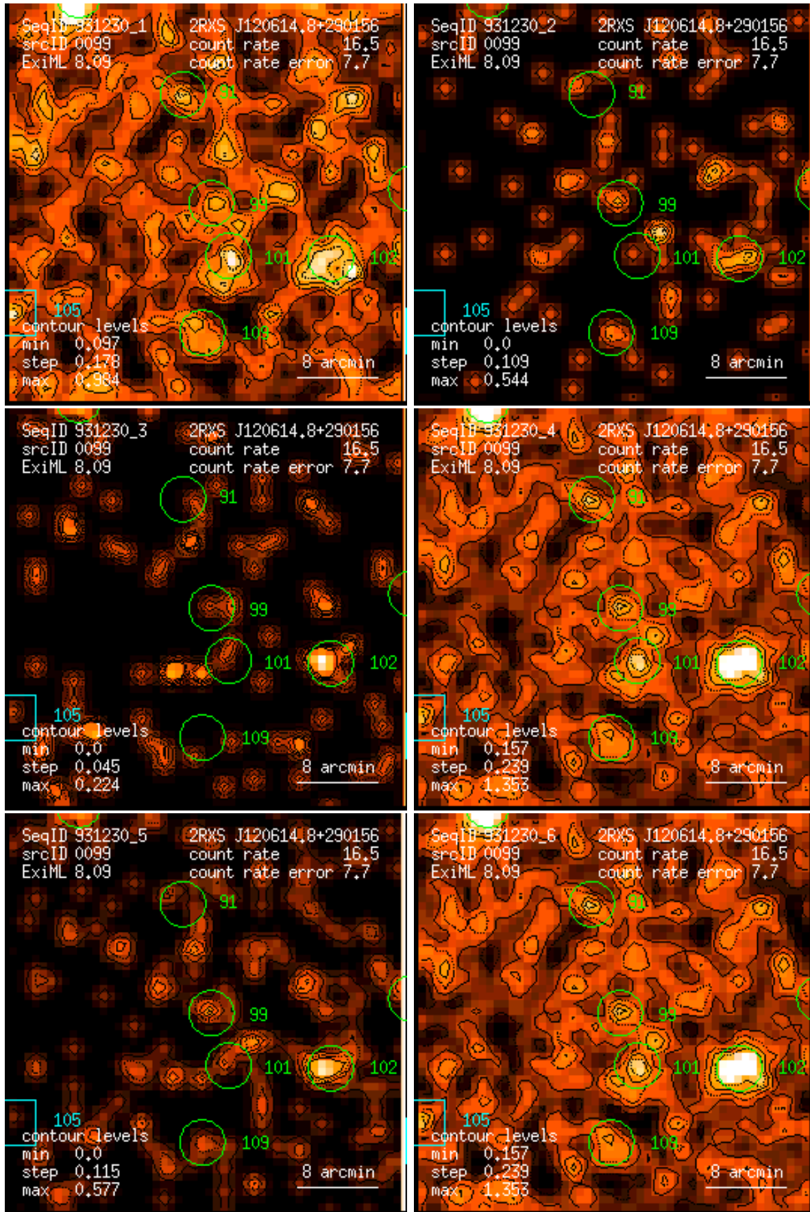
Figure 99: RASS 931230: detection 0099: band rate images, Gaussian filter: (1) PSPC channels 11 – 41, (2) 52 – 90, (3) 91 – 201, (4) 11 – 235, (5) 52 – 201, (6) 11 – 201. Broad band rates in counts/ks. Band rate contour levels in counts/ks/arcmin 2 .
