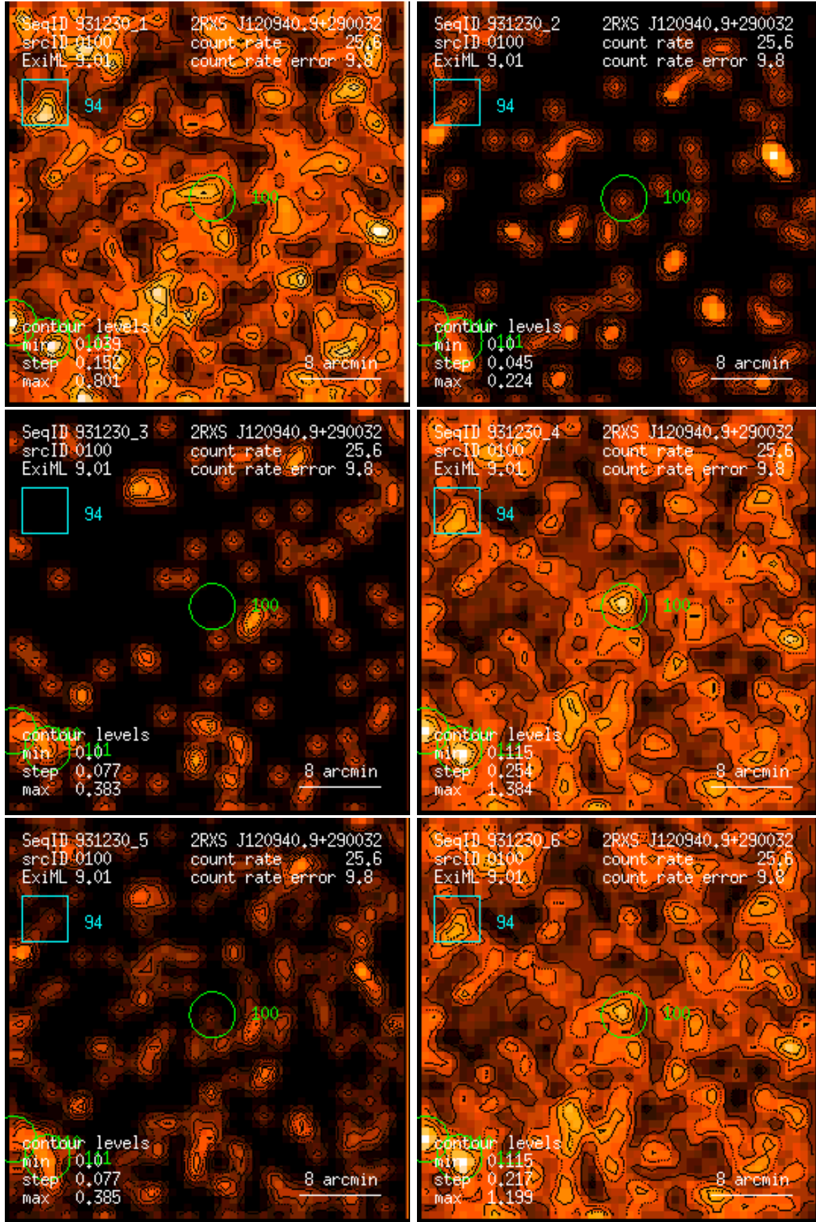
Figure 100: RASS 931230: detection 0100: band rate images, Gaussian filter: (1) PSPC channels 11 – 41, (2) 52 – 90, (3) 91 – 201, (4) 11 – 235, (5) 52 – 201, (6) 11 – 201. Broad band rates in counts/ks. Band rate contour levels in counts/ks/arcmin 2 .
