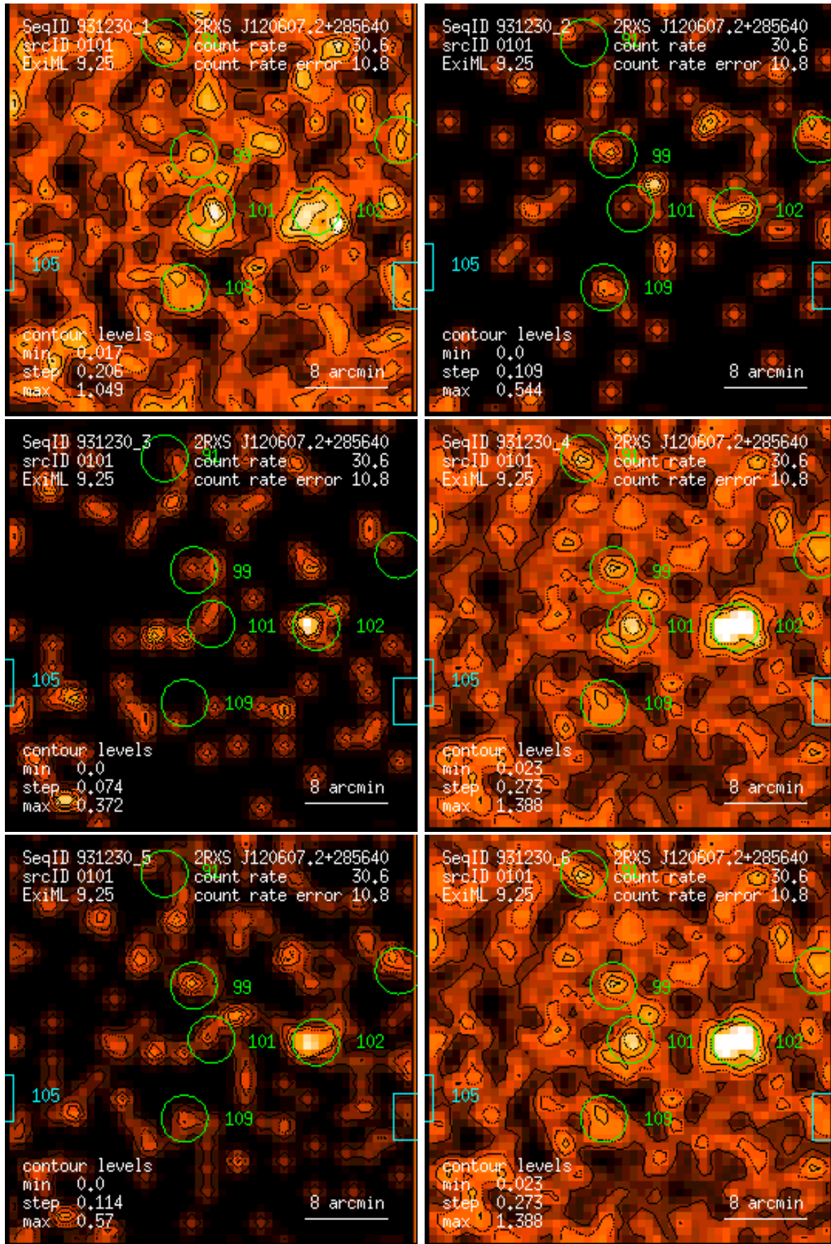
Figure 101: RASS 931230: detection 0101: band rate images, Gaussian filter: (1) PSPC channels 11 – 41, (2) 52 – 90, (3) 91 – 201, (4) 11 – 235, (5) 52 – 201, (6) 11 – 201. Broad band rates in counts/ks. Band rate contour levels in counts/ks/arcmin 2 .
