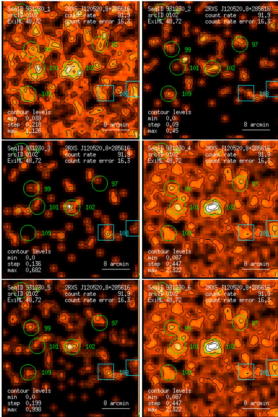
Figure 102: RASS 931230: detection 0102: band rate images, Gaussian filter: (1) PSPC channels 11 – 41, (2) 52 – 90, (3) 91 – 201, (4) 11 – 235, (5) 52 – 201, (6) 11 – 201. Broad band rates in counts/ks. Band rate contour levels in counts/ks/arcmin 2 .
