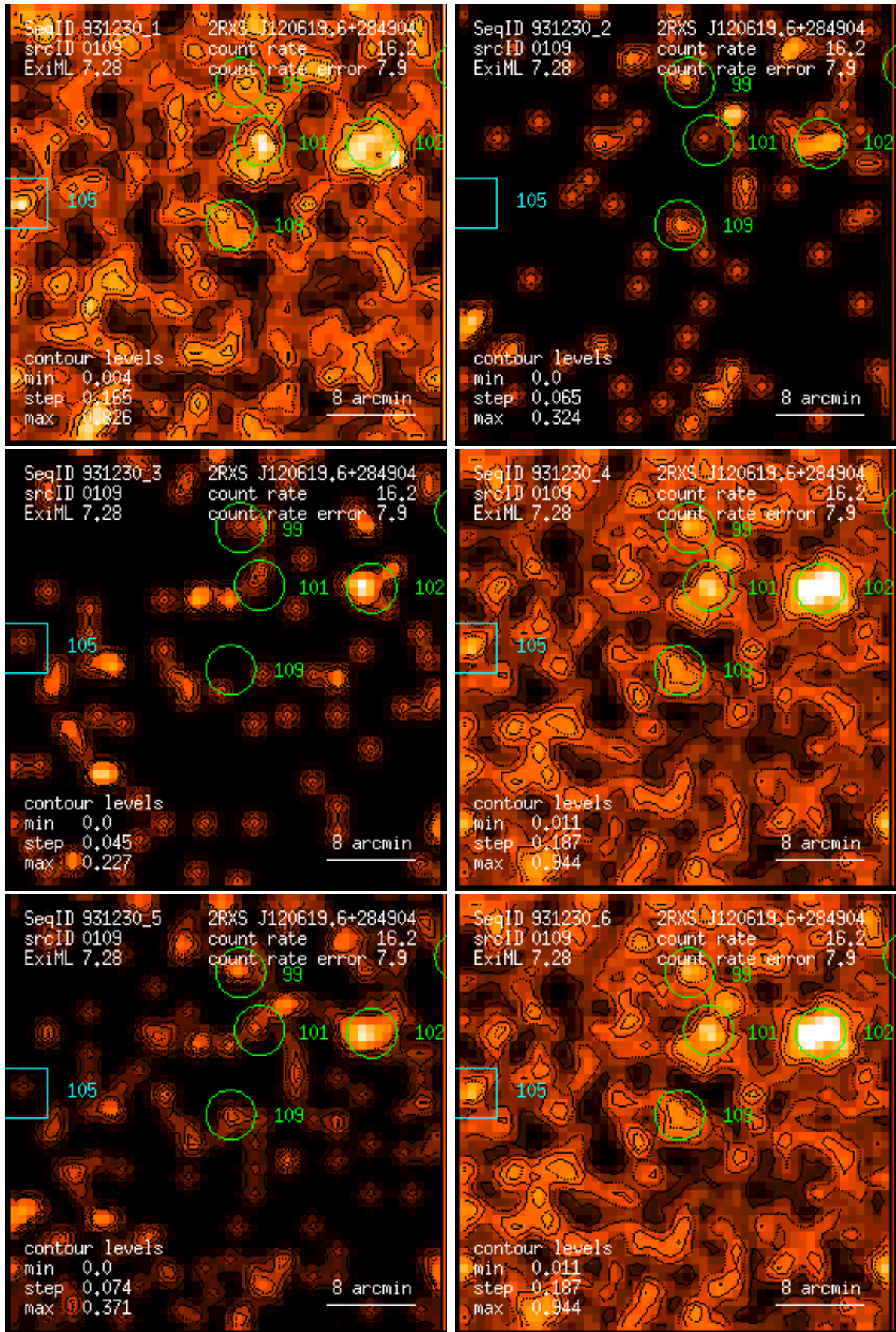
Figure 109: RASS 931230: detection 0109: band rate images, Gaussian filter: (1) PSPC channels 11 – 41, (2) 52 – 90, (3) 91 – 201, (4) 11 – 235, (5) 52 – 201, (6) 11 – 201. Broad band rates in counts/ks. Band rate contour levels in counts/ks/arcmin 2 .
