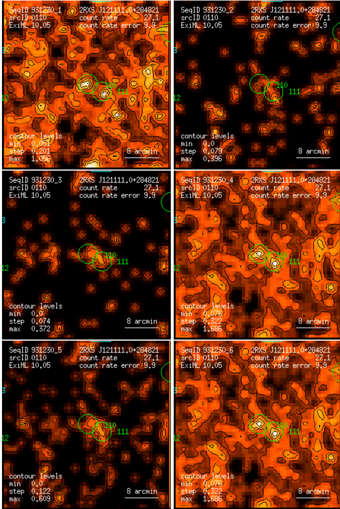
Figure 110: RASS 931230: detection 0110: band rate images, Gaussian filter: (1) PSPC channels 11 – 41, (2) 52 – 90, (3) 91 – 201, (4) 11 – 235, (5) 52 – 201, (6) 11 – 201. Broad band rates in counts/ks. Band rate contour levels in counts/ks/arcmin 2 .
