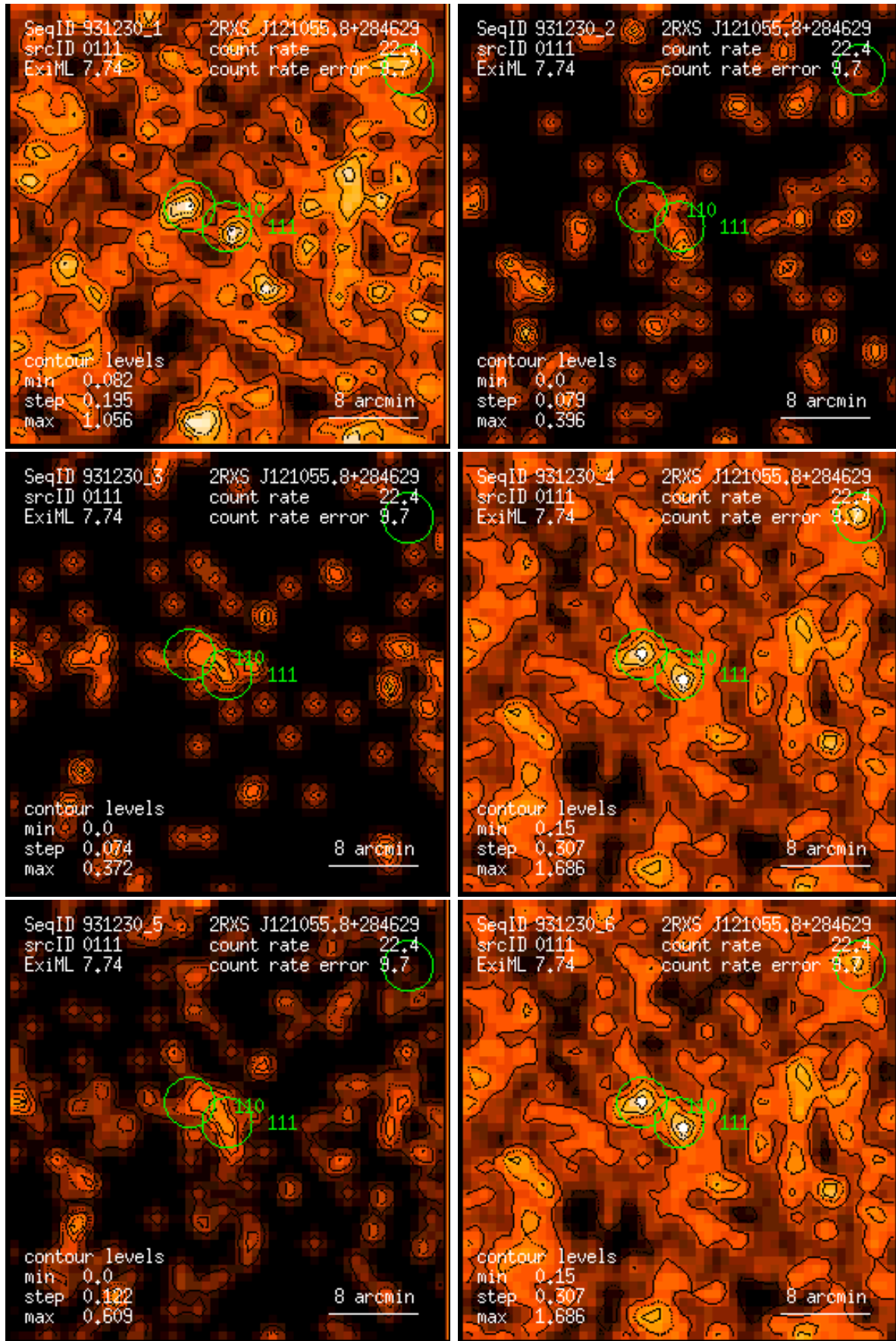
Figure 111: RASS 931230: detection 0111: band rate images, Gaussian filter: (1) PSPC channels 11 – 41, (2) 52 – 90, (3) 91 – 201, (4) 11 – 235, (5) 52 – 201, (6) 11 – 201. Broad band rates in counts/ks. Band rate contour levels in counts/ks/arcmin 2 .
