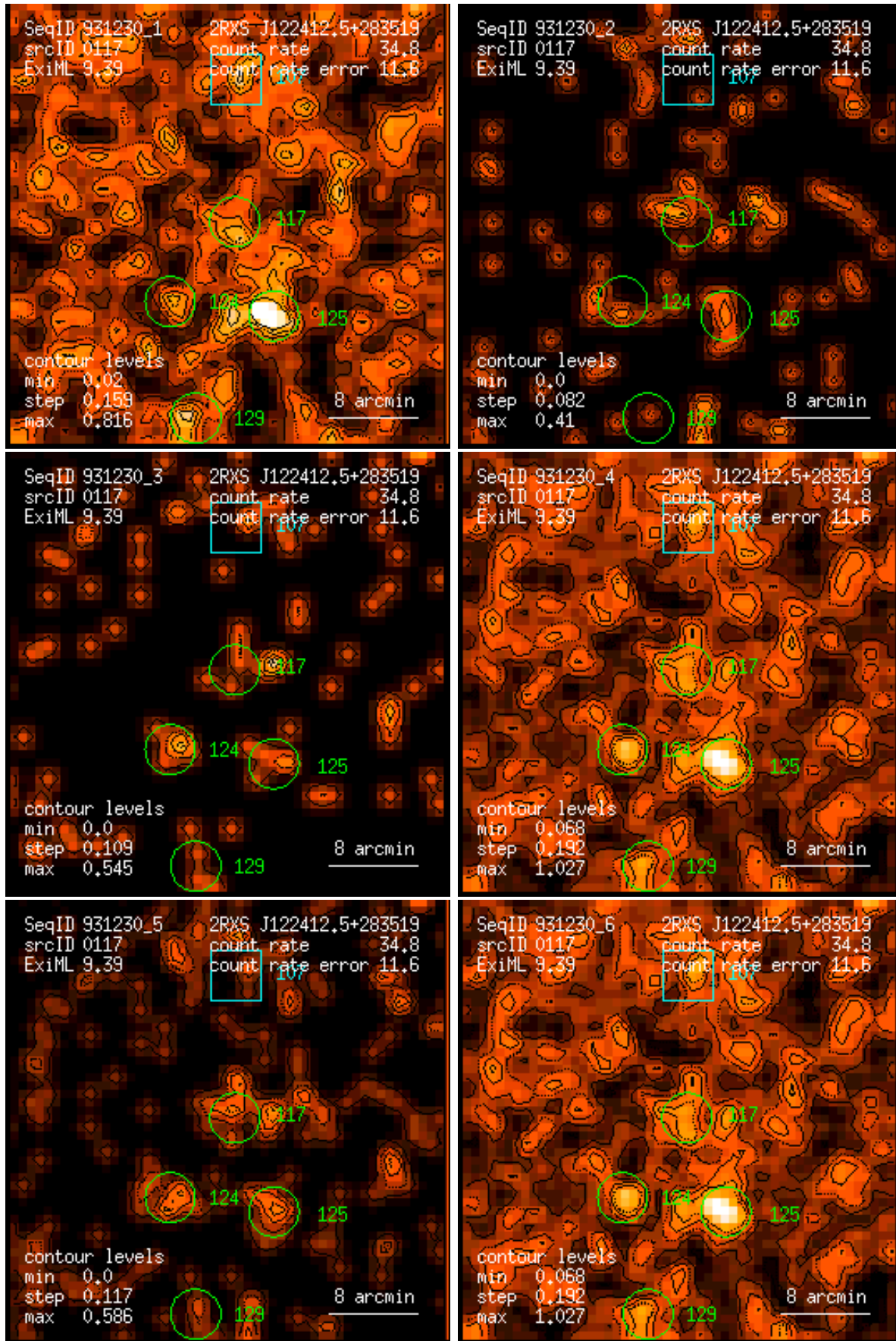
Figure 117: RASS 931230: detection 0117: band rate images, Gaussian filter: (1) PSPC channels 11 – 41, (2) 52 – 90, (3) 91 – 201, (4) 11 – 235, (5) 52 – 201, (6) 11 – 201. Broad band rates in counts/ks. Band rate contour levels in counts/ks/arcmin 2 .
