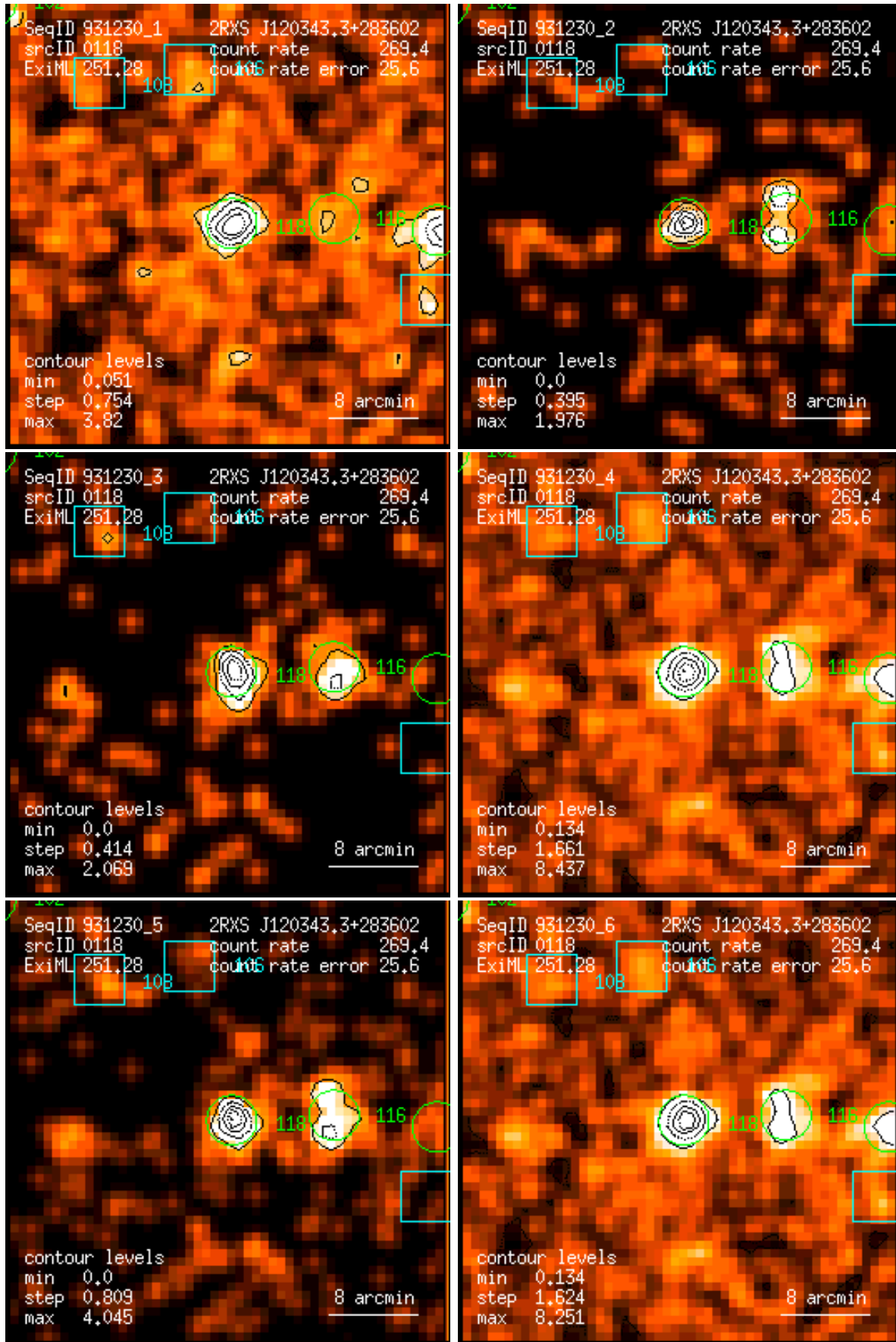
Figure 118: RASS 931230: detection 0118: band rate images, Gaussian filter: (1) PSPC channels 11 – 41, (2) 52 – 90, (3) 91 – 201, (4) 11 – 235, (5) 52 – 201, (6) 11 – 201. Broad band rates in counts/ks. Band rate contour levels in counts/ks/arcmin 2 .
