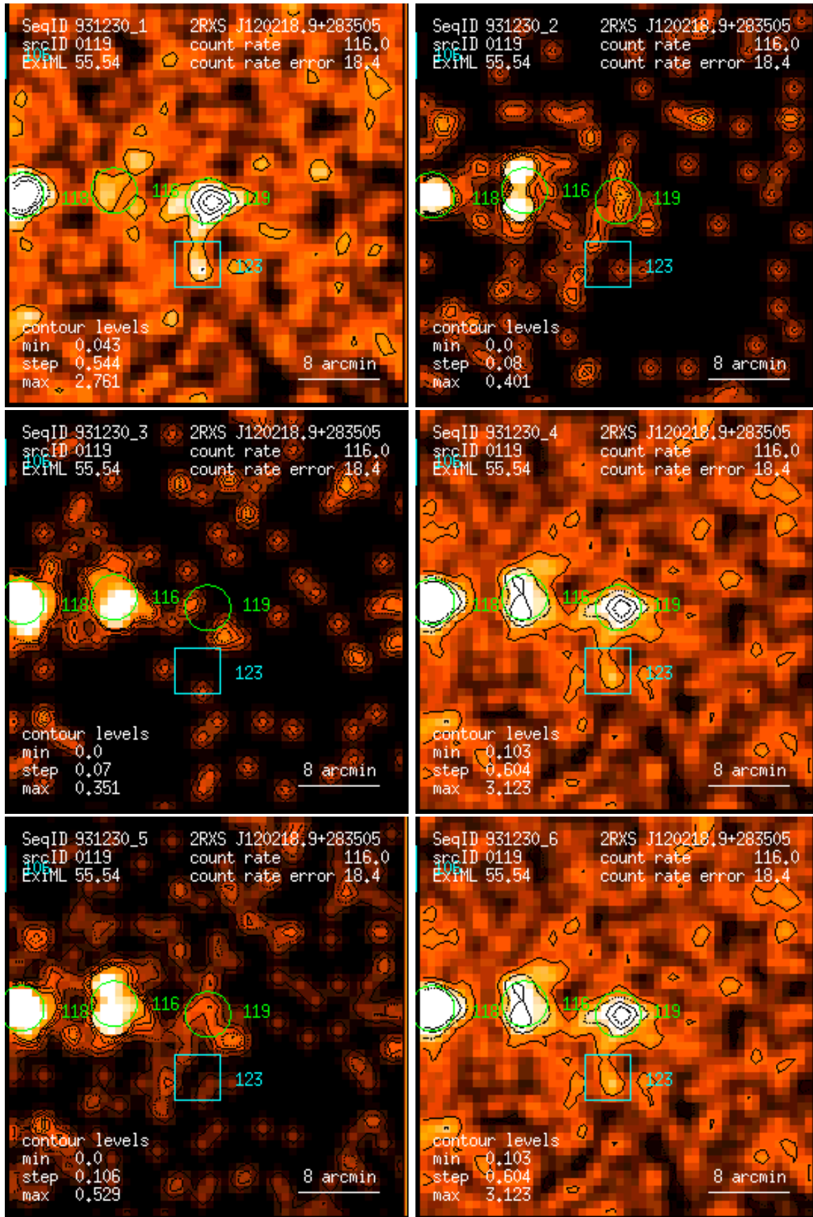
Figure 119: RASS 931230: detection 0119: band rate images, Gaussian filter: (1) PSPC channels 11 – 41, (2) 52 – 90, (3) 91 – 201, (4) 11 – 235, (5) 52 – 201, (6) 11 – 201. Broad band rates in counts/ks. Band rate contour levels in counts/ks/arcmin 2 .
