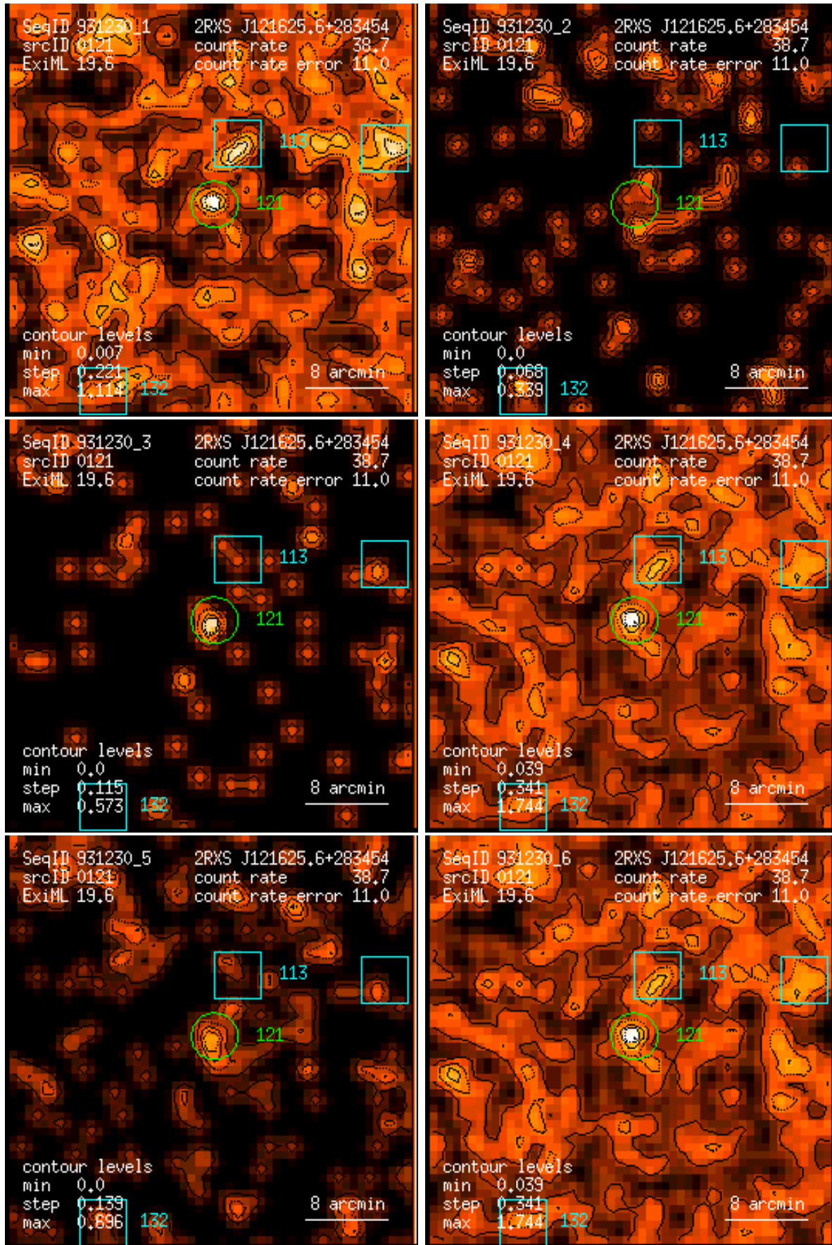
Figure 121: RASS 931230: detection 0121: band rate images, Gaussian filter: (1) PSPC channels 11 – 41, (2) 52 – 90, (3) 91 – 201, (4) 11 – 235, (5) 52 – 201, (6) 11 – 201. Broad band rates in counts/ks. Band rate contour levels in counts/ks/arcmin 2 .
