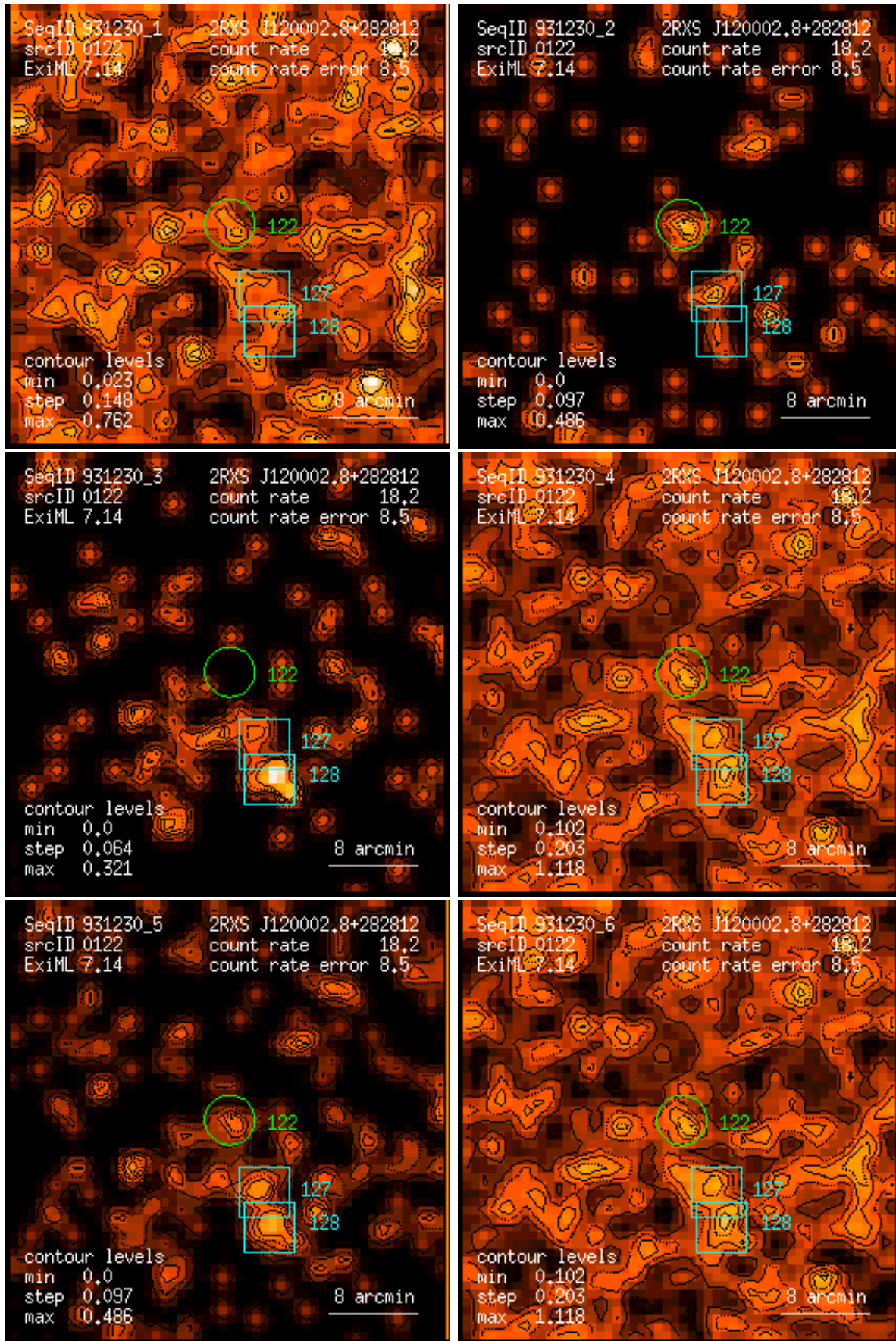
Figure 122: RASS 931230: detection 0122: band rate images, Gaussian filter: (1) PSPC channels 11 – 41, (2) 52 – 90, (3) 91 – 201, (4) 11 – 235, (5) 52 – 201, (6) 11 – 201. Broad band rates in counts/ks. Band rate contour levels in counts/ks/arcmin 2 .
