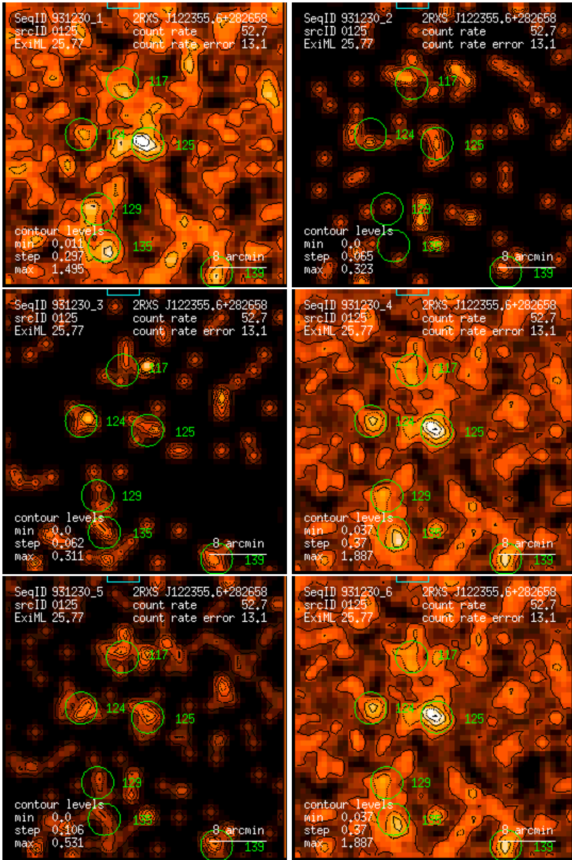
Figure 125: RASS 931230: detection 0125: band rate images, Gaussian filter: (1) PSPC channels 11 – 41, (2) 52 – 90, (3) 91 – 201, (4) 11 – 235, (5) 52 – 201, (6) 11 – 201. Broad band rates in counts/ks. Band rate contour levels in counts/ks/arcmin 2 .
