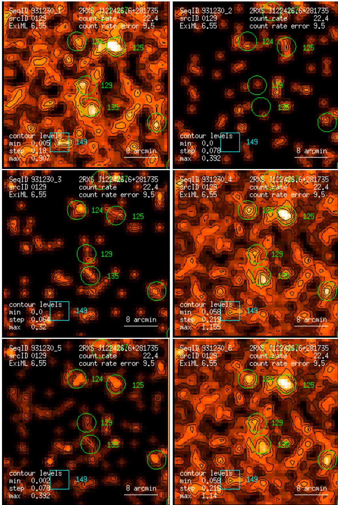
Figure 129: RASS 931230: detection 0129: band rate images, Gaussian filter: (1) PSPC channels 11 – 41, (2) 52 – 90, (3) 91 – 201, (4) 11 – 235, (5) 52 – 201, (6) 11 – 201. Broad band rates in counts/ks. Band rate contour levels in counts/ks/arcmin 2 .
