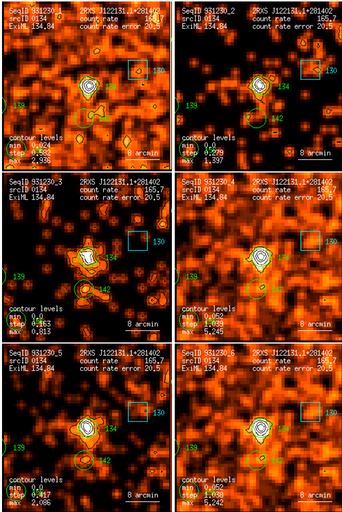
Figure 134: RASS 931230: detection 0134: band rate images, Gaussian filter: (1) PSPC channels 11 – 41, (2) 52 – 90, (3) 91 – 201, (4) 11 – 235, (5) 52 – 201, (6) 11 – 201. Broad band rates in counts/ks. Band rate contour levels in counts/ks/arcmin 2 .
