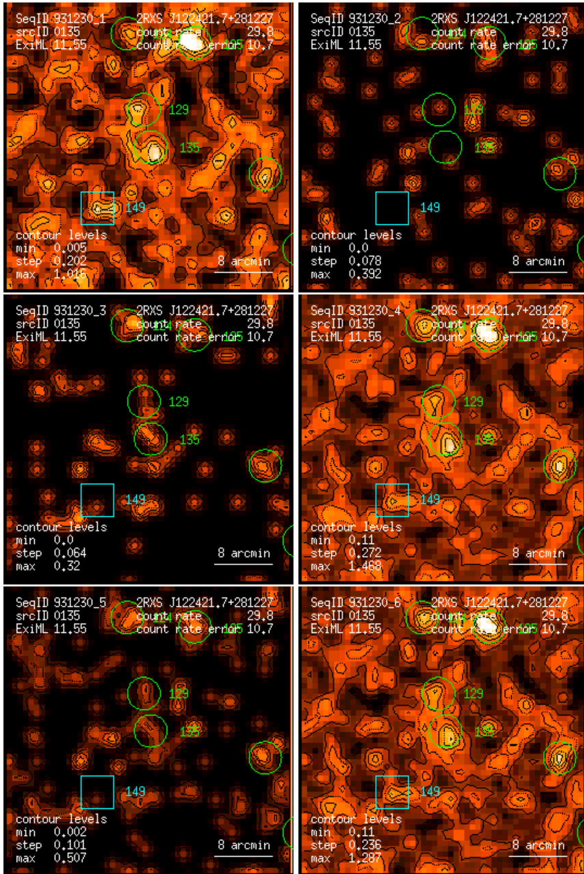
Figure 135: RASS 931230: detection 0135: band rate images, Gaussian filter: (1) PSPC channels 11 – 41, (2) 52 – 90, (3) 91 – 201, (4) 11 – 235, (5) 52 – 201, (6) 11 – 201. Broad band rates in counts/ks. Band rate contour levels in counts/ks/arcmin 2 .
