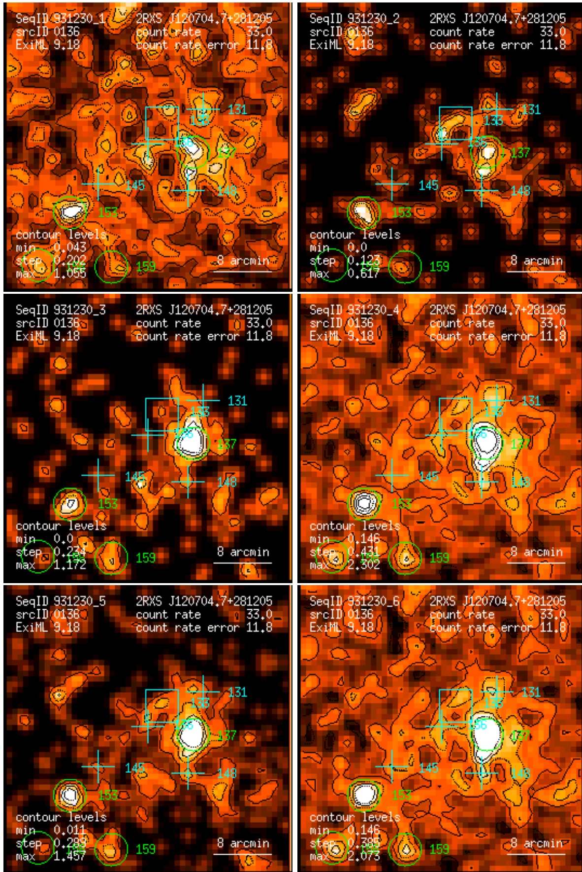
Figure 136: RASS 931230: detection 0136: band rate images, Gaussian filter: (1) PSPC channels 11 – 41, (2) 52 – 90, (3) 91 – 201, (4) 11 – 235, (5) 52 – 201, (6) 11 – 201. Broad band rates in counts/ks. Band rate contour levels in counts/ks/arcmin 2 .
