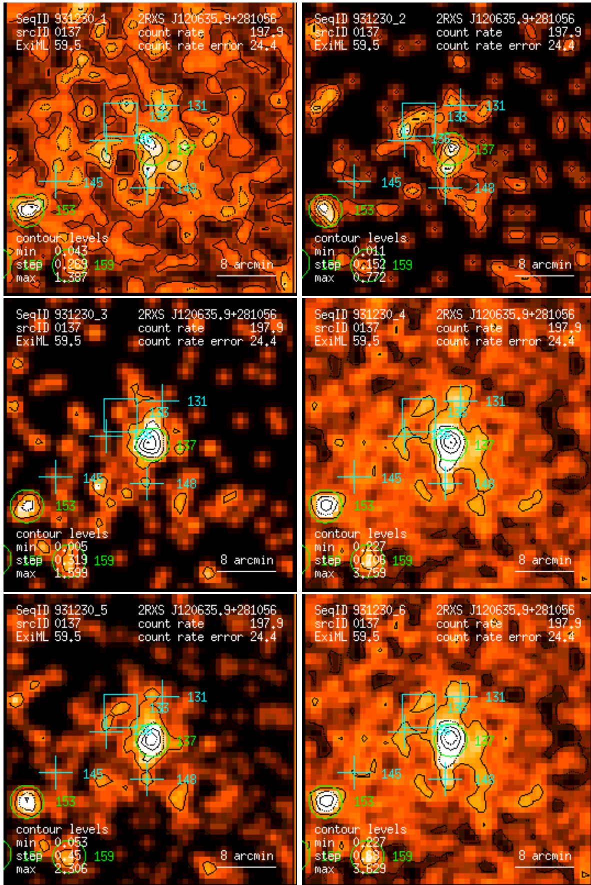
Figure 137: RASS 931230: detection 0137: band rate images, Gaussian filter: (1) PSPC channels 11 – 41, (2) 52 – 90, (3) 91 – 201, (4) 11 – 235, (5) 52 – 201, (6) 11 – 201. Broad band rates in counts/ks. Band rate contour levels in counts/ks/arcmin 2 .
