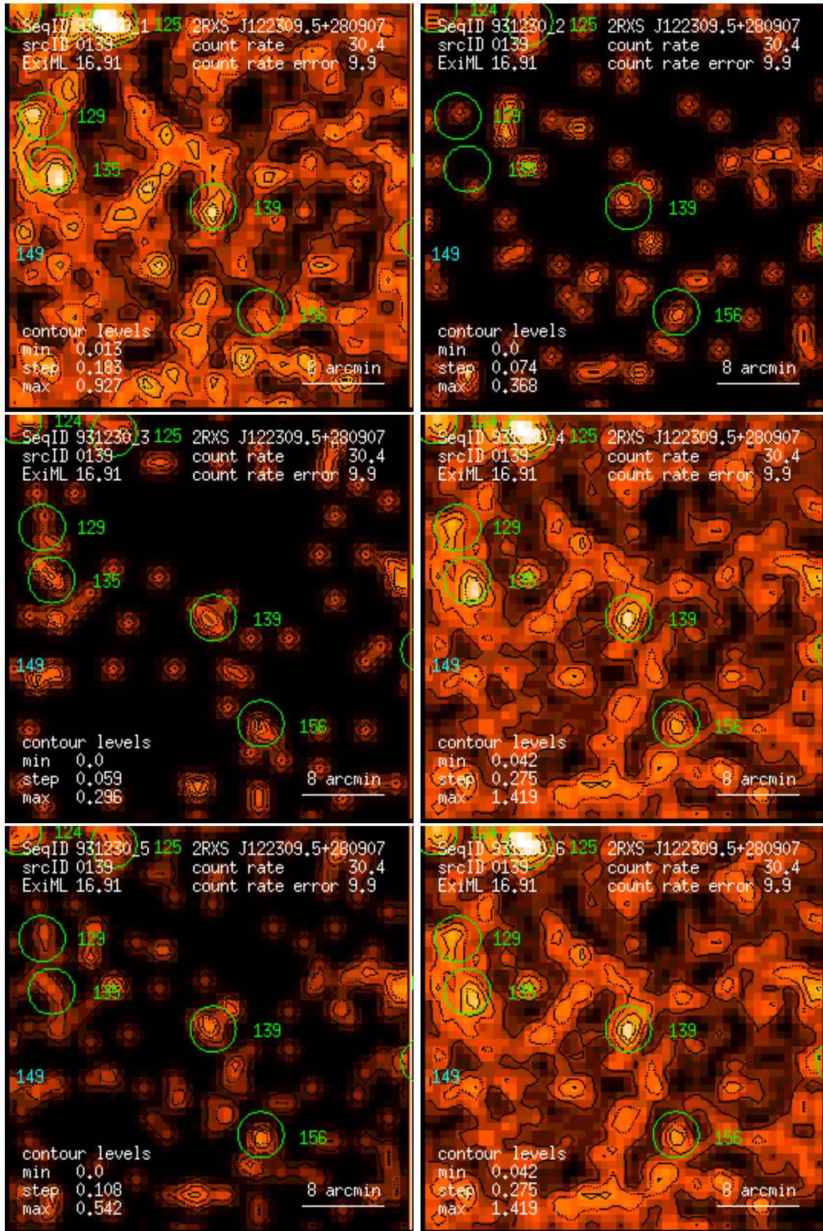
Figure 139: RASS 931230: detection 0139: band rate images, Gaussian filter: (1) PSPC channels 11 – 41, (2) 52 – 90, (3) 91 – 201, (4) 11 – 235, (5) 52 – 201, (6) 11 – 201. Broad band rates in counts/ks. Band rate contour levels in counts/ks/arcmin 2 .
