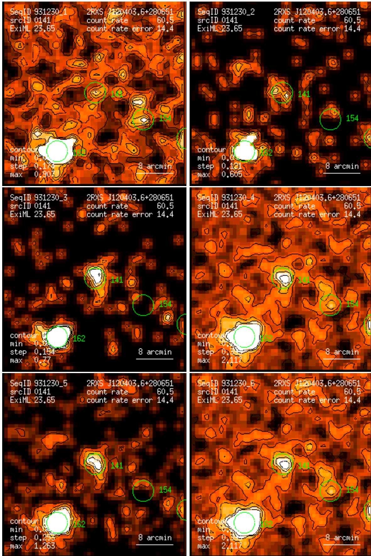
Figure 141: RASS 931230: detection 0141: band rate images, Gaussian filter: (1) PSPC channels 11 – 41, (2) 52 – 90, (3) 91 – 201, (4) 11 – 235, (5) 52 – 201, (6) 11 – 201. Broad band rates in counts/ks. Band rate contour levels in counts/ks/arcmin 2 .
