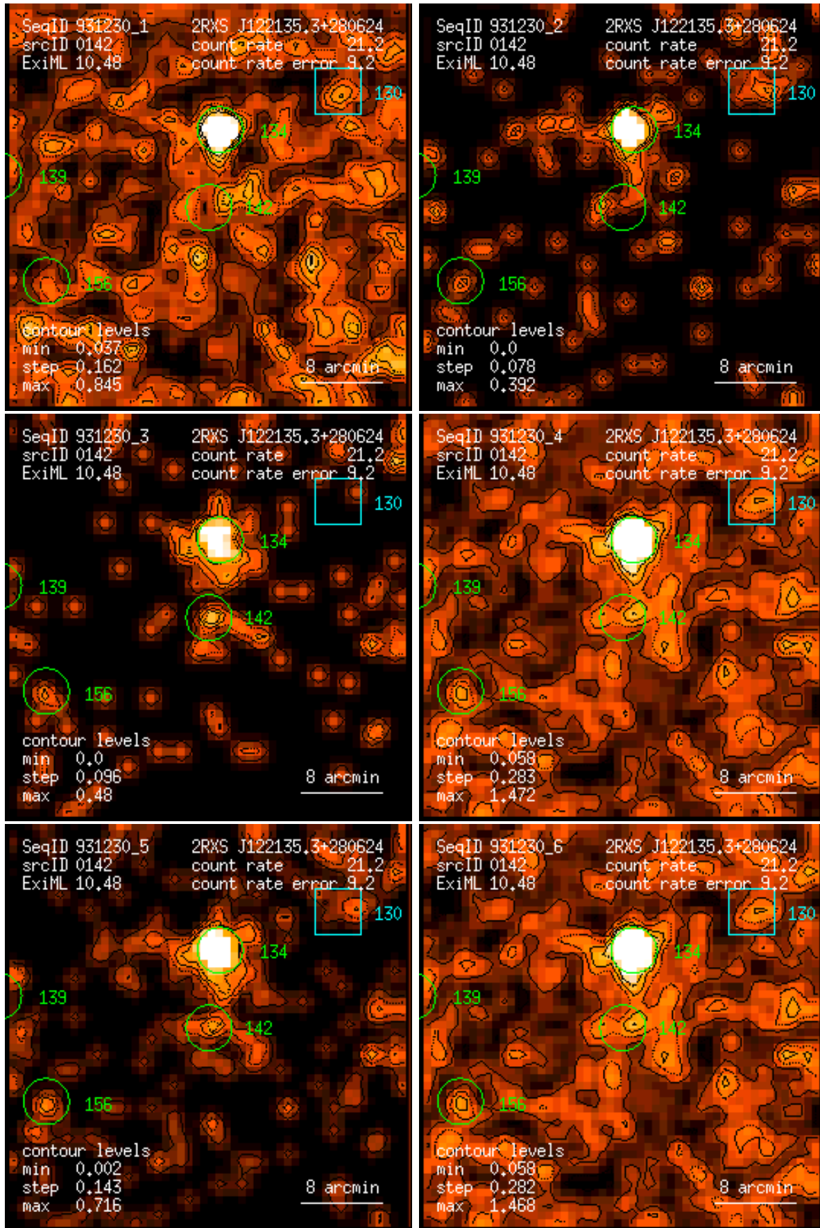
Figure 142: RASS 931230: detection 0142: band rate images, Gaussian filter: (1) PSPC channels 11 – 41, (2) 52 – 90, (3) 91 – 201, (4) 11 – 235, (5) 52 – 201, (6) 11 – 201. Broad band rates in counts/ks. Band rate contour levels in counts/ks/arcmin 2 .
