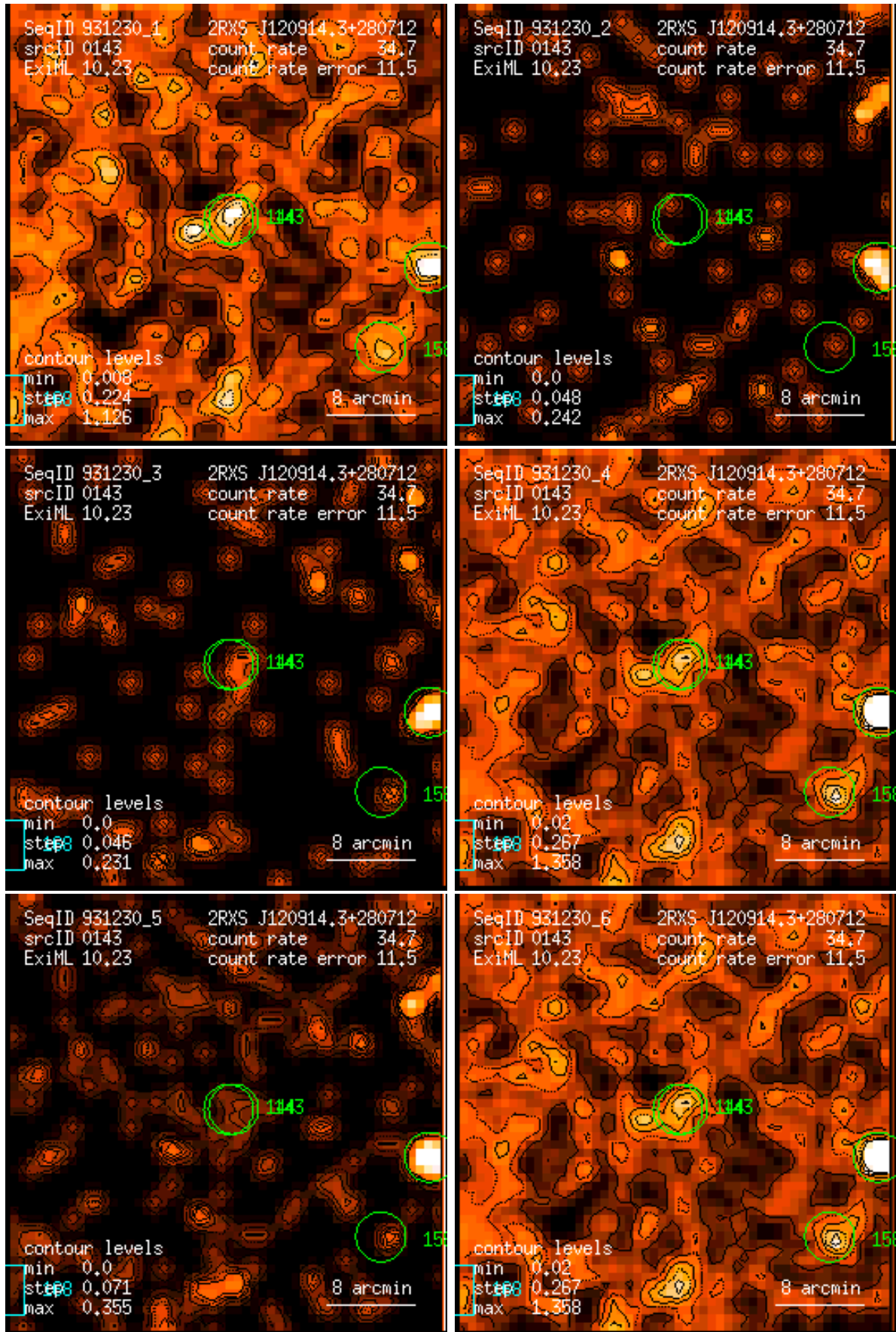
Figure 143: RASS 931230: detection 0143: band rate images, Gaussian filter: (1) PSPC channels 11 – 41, (2) 52 – 90, (3) 91 – 201, (4) 11 – 235, (5) 52 – 201, (6) 11 – 201. Broad band rates in counts/ks. Band rate contour levels in counts/ks/arcmin 2 .
