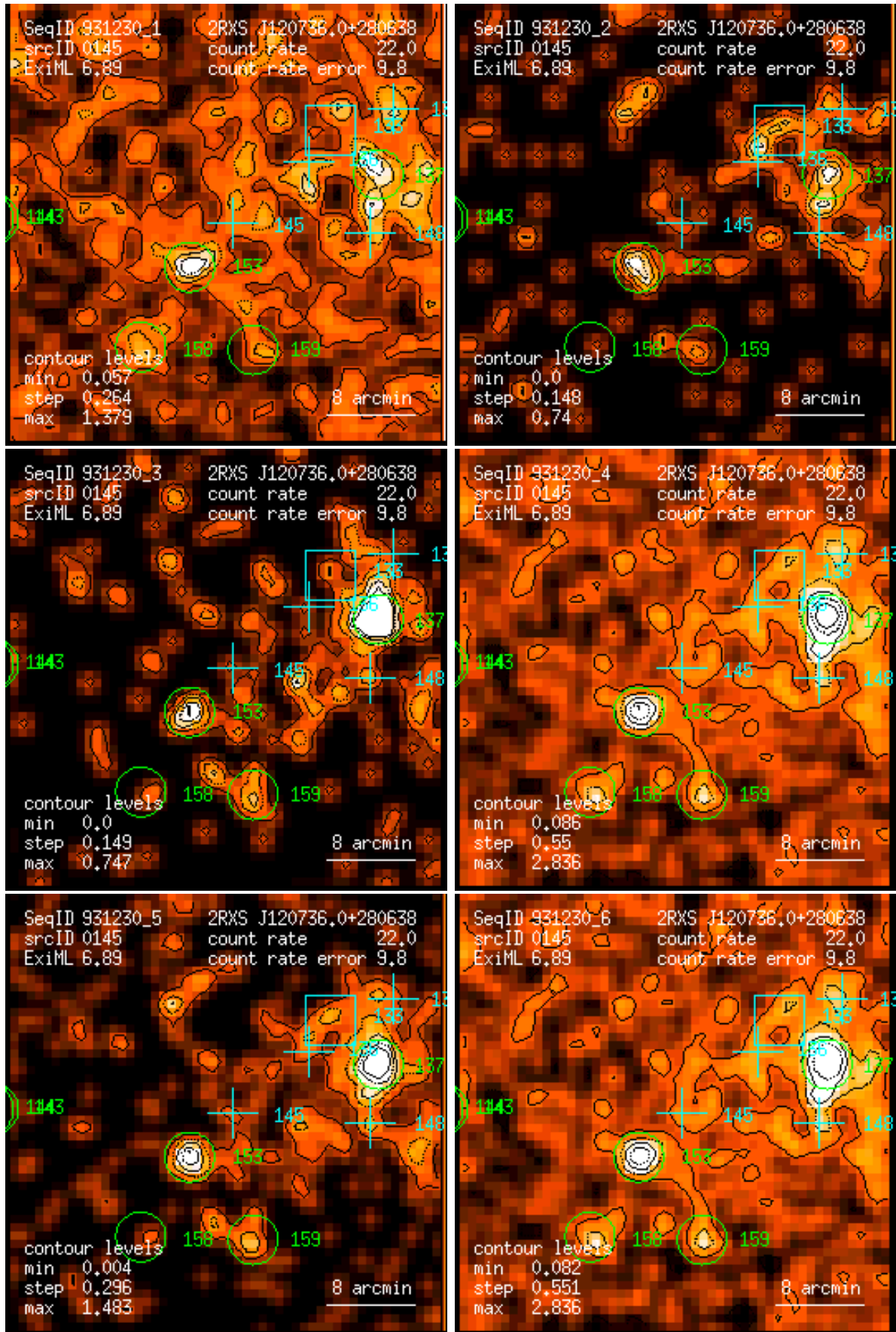
Figure 145: RASS 931230: detection 0145: band rate images, Gaussian filter: (1) PSPC channels 11 – 41, (2) 52 – 90, (3) 91 – 201, (4) 11 – 235, (5) 52 – 201, (6) 11 – 201. Broad band rates in counts/ks. Band rate contour levels in counts/ks/arcmin 2 .
