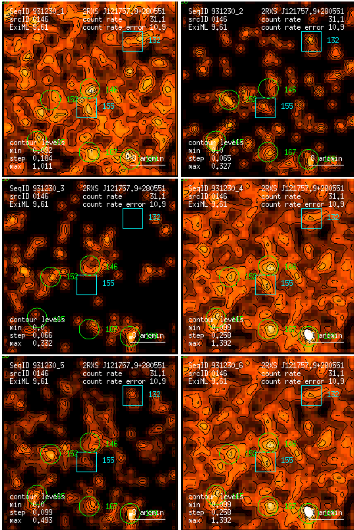
Figure 146: RASS 931230: detection 0146: band rate images, Gaussian filter: (1) PSPC channels 11 – 41, (2) 52 – 90, (3) 91 – 201, (4) 11 – 235, (5) 52 – 201, (6) 11 – 201. Broad band rates in counts/ks. Band rate contour levels in counts/ks/arcmin 2 .
