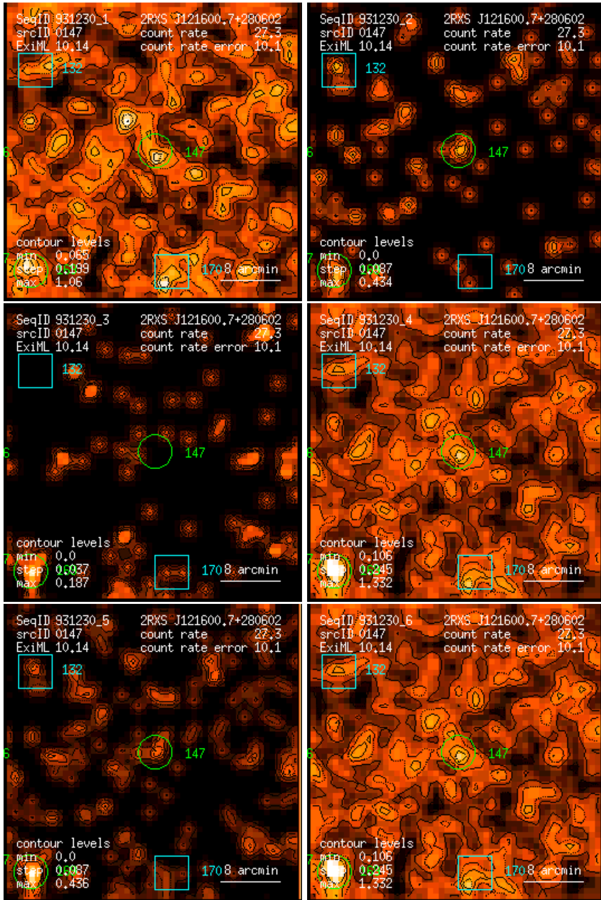
Figure 147: RASS 931230: detection 0147: band rate images, Gaussian filter: (1) PSPC channels 11 – 41, (2) 52 – 90, (3) 91 – 201, (4) 11 – 235, (5) 52 – 201, (6) 11 – 201. Broad band rates in counts/ks. Band rate contour levels in counts/ks/arcmin 2 .
