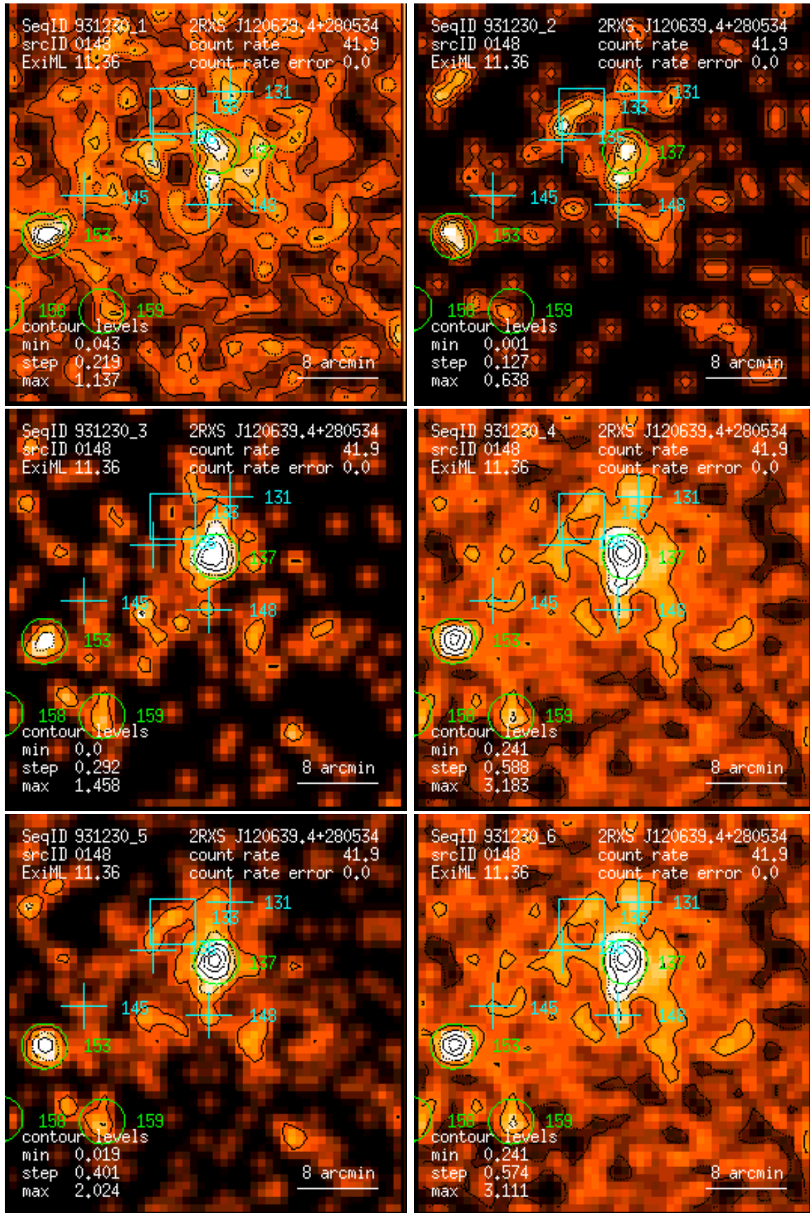
Figure 148: RASS 931230: detection 0148: band rate images, Gaussian filter: (1) PSPC channels 11 – 41, (2) 52 – 90, (3) 91 – 201, (4) 11 – 235, (5) 52 – 201, (6) 11 – 201. Broad band rates in counts/ks. Band rate contour levels in counts/ks/arcmin 2 .
