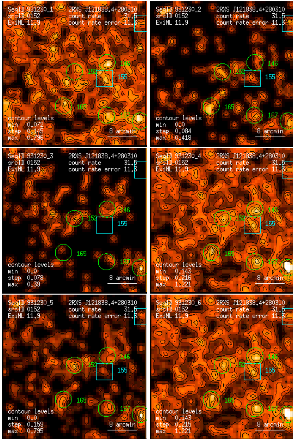
Figure 152: RASS 931230: detection 0152: band rate images, Gaussian filter: (1) PSPC channels 11 – 41, (2) 52 – 90, (3) 91 – 201, (4) 11 – 235, (5) 52 – 201, (6) 11 – 201. Broad band rates in counts/ks. Band rate contour levels in counts/ks/arcmin 2 .
