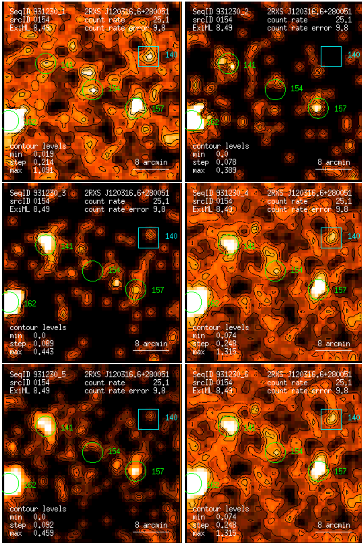
Figure 154: RASS 931230: detection 0154: band rate images, Gaussian filter: (1) PSPC channels 11 – 41, (2) 52 – 90, (3) 91 – 201, (4) 11 – 235, (5) 52 – 201, (6) 11 – 201. Broad band rates in counts/ks. Band rate contour levels in counts/ks/arcmin 2 .
