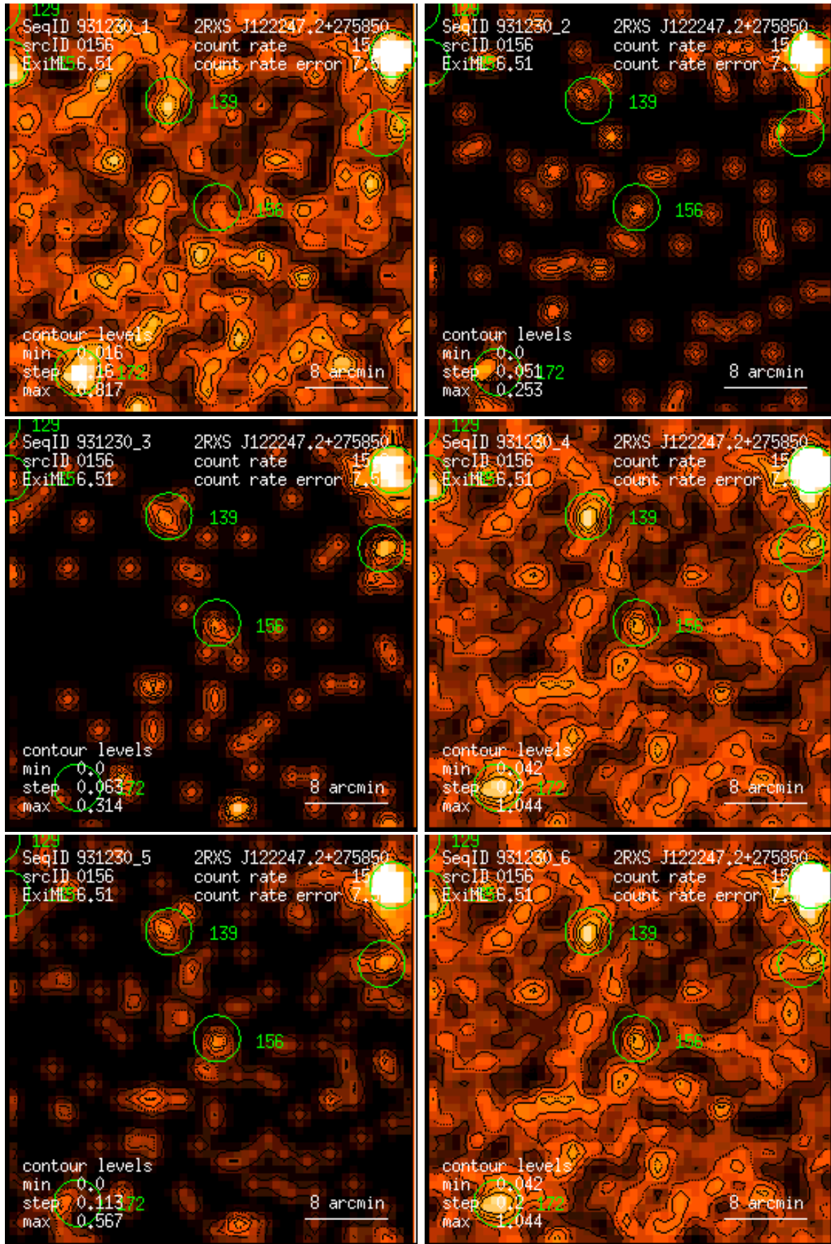
Figure 156: RASS 931230: detection 0156: band rate images, Gaussian filter: (1) PSPC channels 11 – 41, (2) 52 – 90, (3) 91 – 201, (4) 11 – 235, (5) 52 – 201, (6) 11 – 201. Broad band rates in counts/ks. Band rate contour levels in counts/ks/arcmin 2 .
