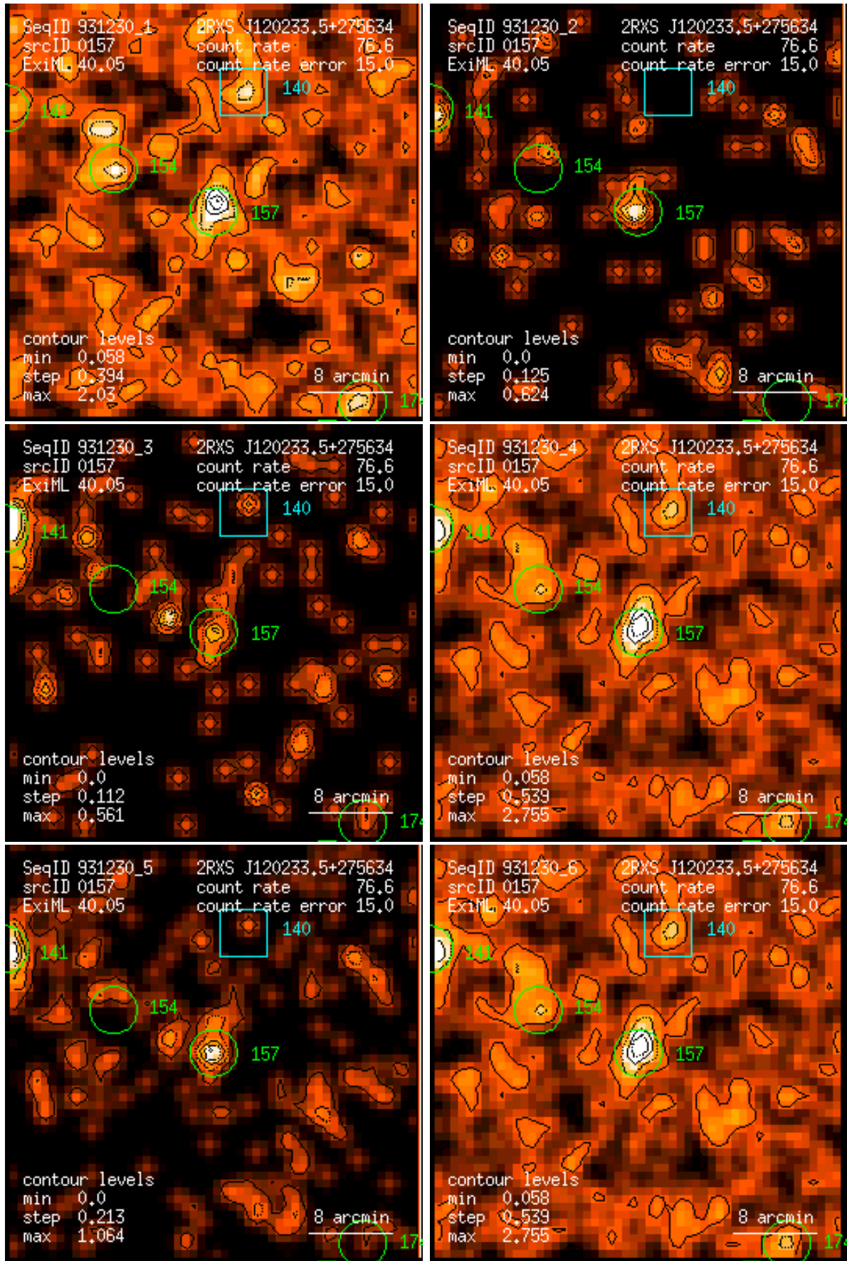
Figure 157: RASS 931230: detection 0157: band rate images, Gaussian filter: (1) PSPC channels 11 – 41, (2) 52 – 90, (3) 91 – 201, (4) 11 – 235, (5) 52 – 201, (6) 11 – 201. Broad band rates in counts/ks. Band rate contour levels in counts/ks/arcmin 2 .
