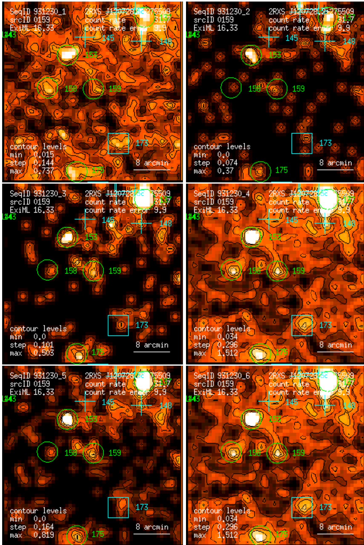
Figure 159: RASS 931230: detection 0159: band rate images, Gaussian filter: (1) PSPC channels 11 – 41, (2) 52 – 90, (3) 91 – 201, (4) 11 – 235, (5) 52 – 201, (6) 11 – 201. Broad band rates in counts/ks. Band rate contour levels in counts/ks/arcmin 2 .
