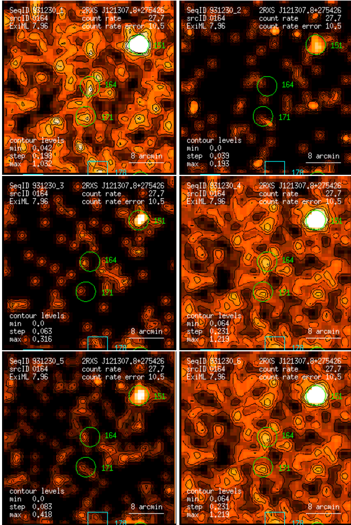
Figure 164: RASS 931230: detection 0164: band rate images, Gaussian filter: (1) PSPC channels 11 – 41, (2) 52 – 90, (3) 91 – 201, (4) 11 – 235, (5) 52 – 201, (6) 11 – 201. Broad band rates in counts/ks. Band rate contour levels in counts/ks/arcmin 2 .
